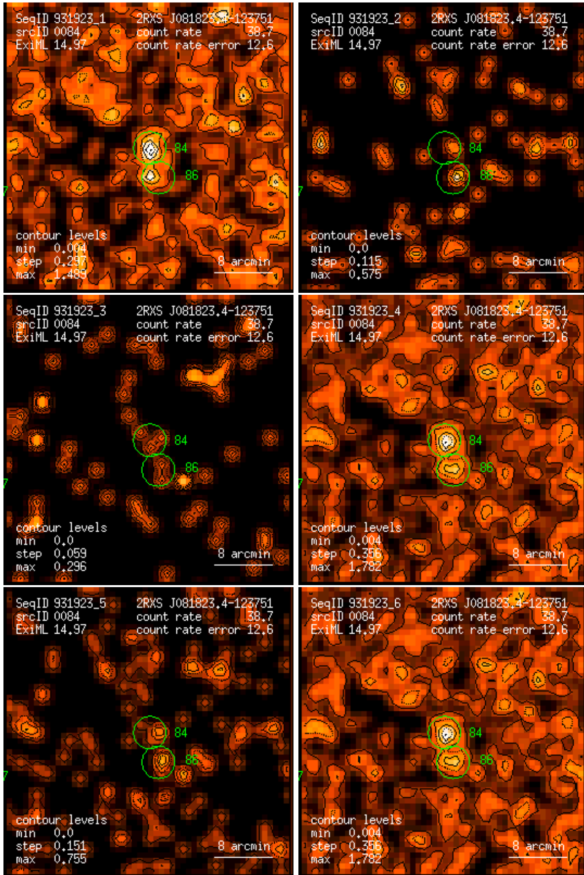
Figure 84: RASS 931923: detection 0084: band rate images, Gaussian filter: (1) PSPC channels 11 – 41, (2) 52 – 90, (3) 91 – 201, (4) 11 – 235, (5) 52 – 201, (6) 11 – 201. Broad band rates in counts/ks. Band rate contour levels in counts/ks/arcmin 2 .
