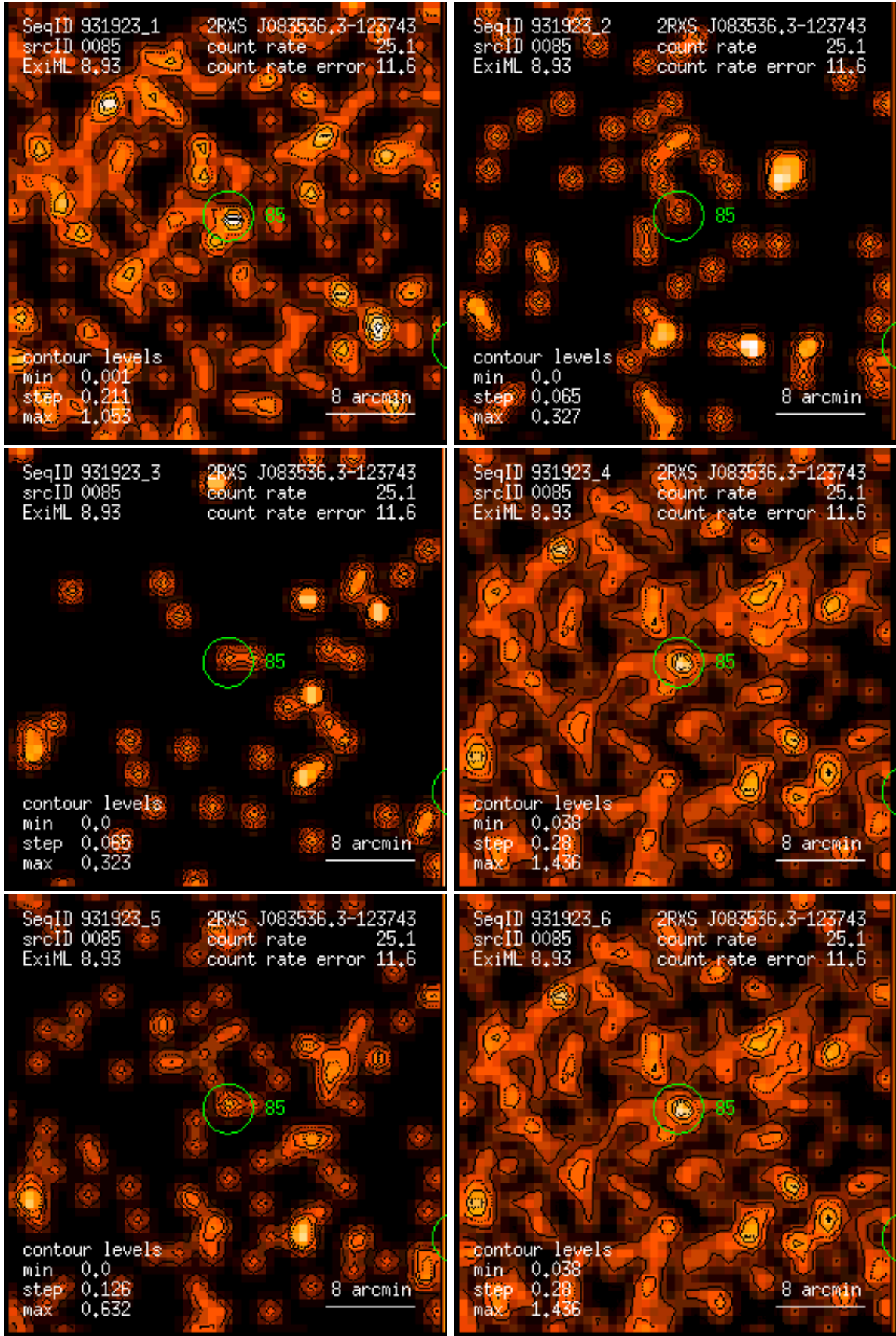
Figure 85: RASS 931923: detection 0085: band rate images, Gaussian filter: (1) PSPC channels 11 – 41, (2) 52 – 90, (3) 91 – 201, (4) 11 – 235, (5) 52 – 201, (6) 11 – 201. Broad band rates in counts/ks. Band rate contour levels in counts/ks/arcmin 2 .
