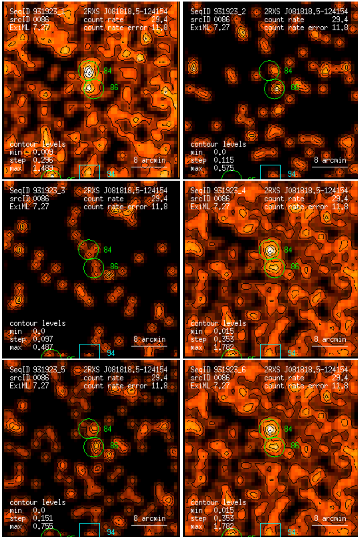
Figure 86: RASS 931923: detection 0086: band rate images, Gaussian filter: (1) PSPC channels 11 – 41, (2) 52 – 90, (3) 91 – 201, (4) 11 – 235, (5) 52 – 201, (6) 11 – 201. Broad band rates in counts/ks. Band rate contour levels in counts/ks/arcmin 2 .
