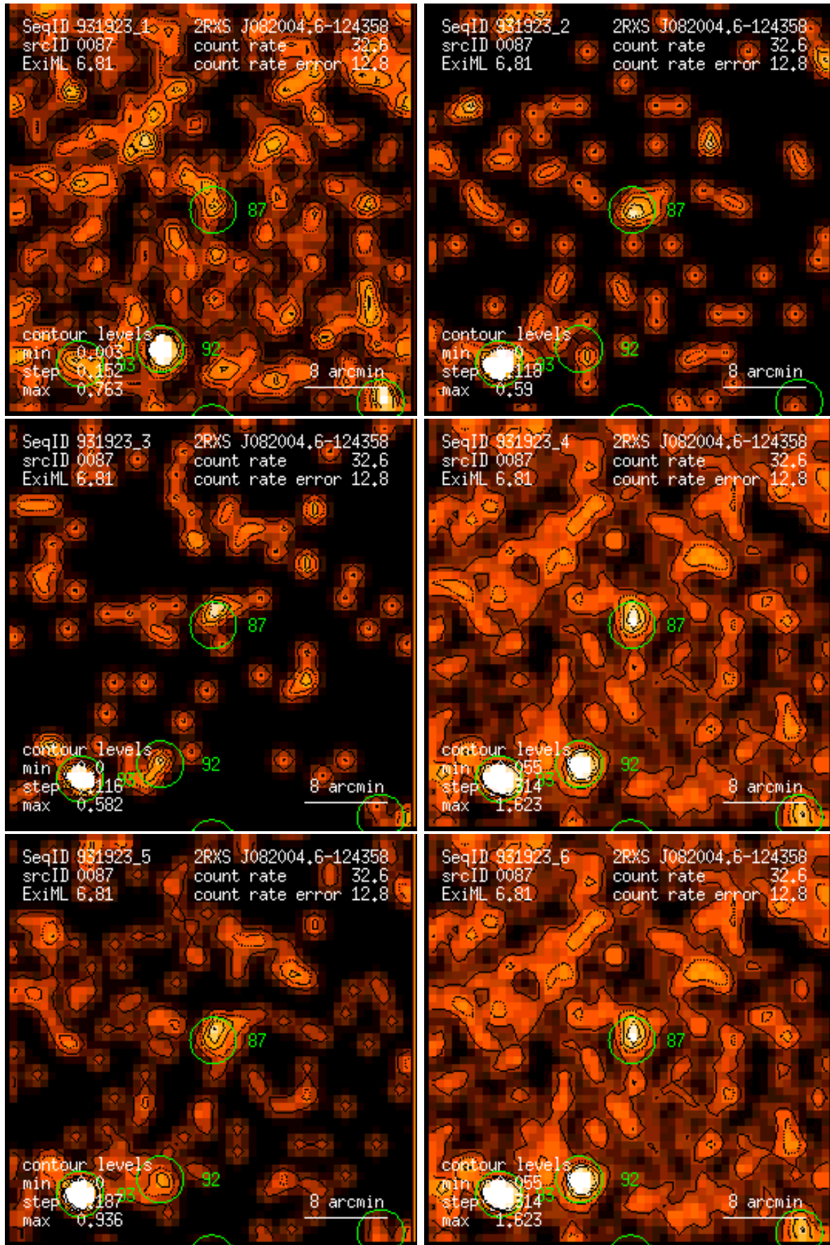
Figure 87: RASS 931923: detection 0087: band rate images, Gaussian filter: (1) PSPC channels 11 – 41, (2) 52 – 90, (3) 91 – 201, (4) 11 – 235, (5) 52 – 201, (6) 11 – 201. Broad band rates in counts/ks. Band rate contour levels in counts/ks/arcmin 2 .
