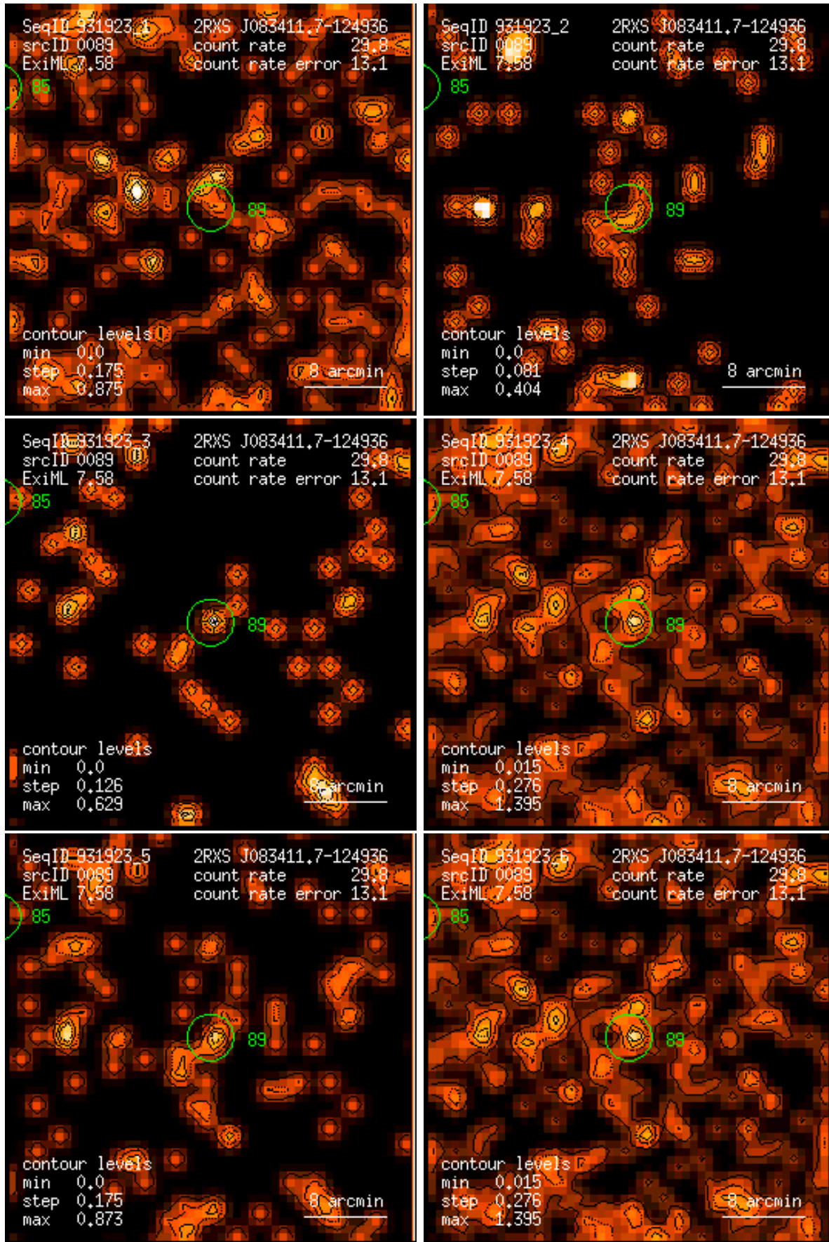
Figure 89: RASS 931923: detection 0089: band rate images, Gaussian filter: (1) PSPC channels 11 – 41, (2) 52 – 90, (3) 91 – 201, (4) 11 – 235, (5) 52 – 201, (6) 11 – 201. Broad band rates in counts/ks. Band rate contour levels in counts/ks/arcmin 2 .
