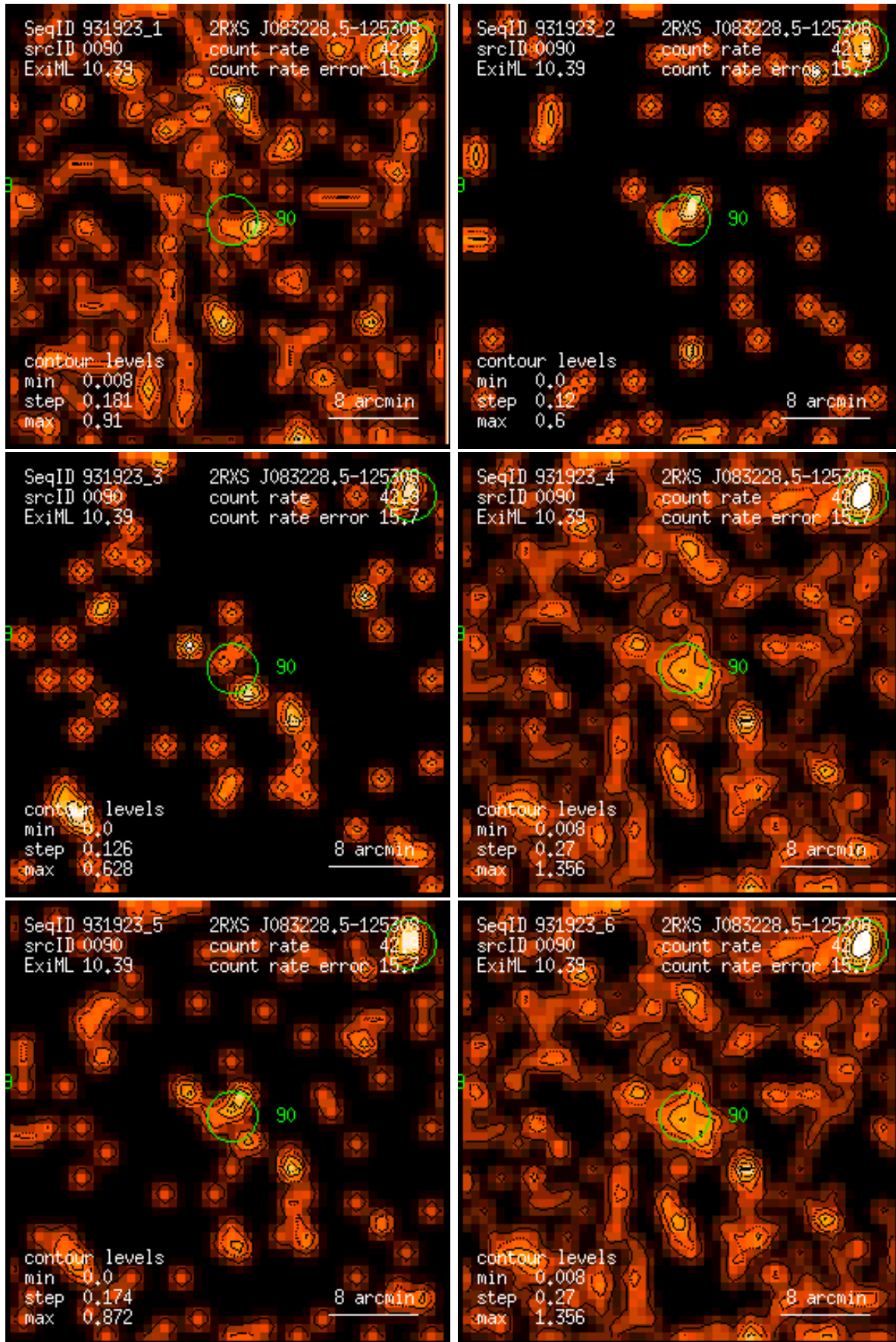
Figure 90: RASS 931923: detection 0090: band rate images, Gaussian filter: (1) PSPC channels 11 – 41, (2) 52 – 90, (3) 91 – 201, (4) 11 – 235, (5) 52 – 201, (6) 11 – 201. Broad band rates in counts/ks. Band rate contour levels in counts/ks/arcmin 2 .
