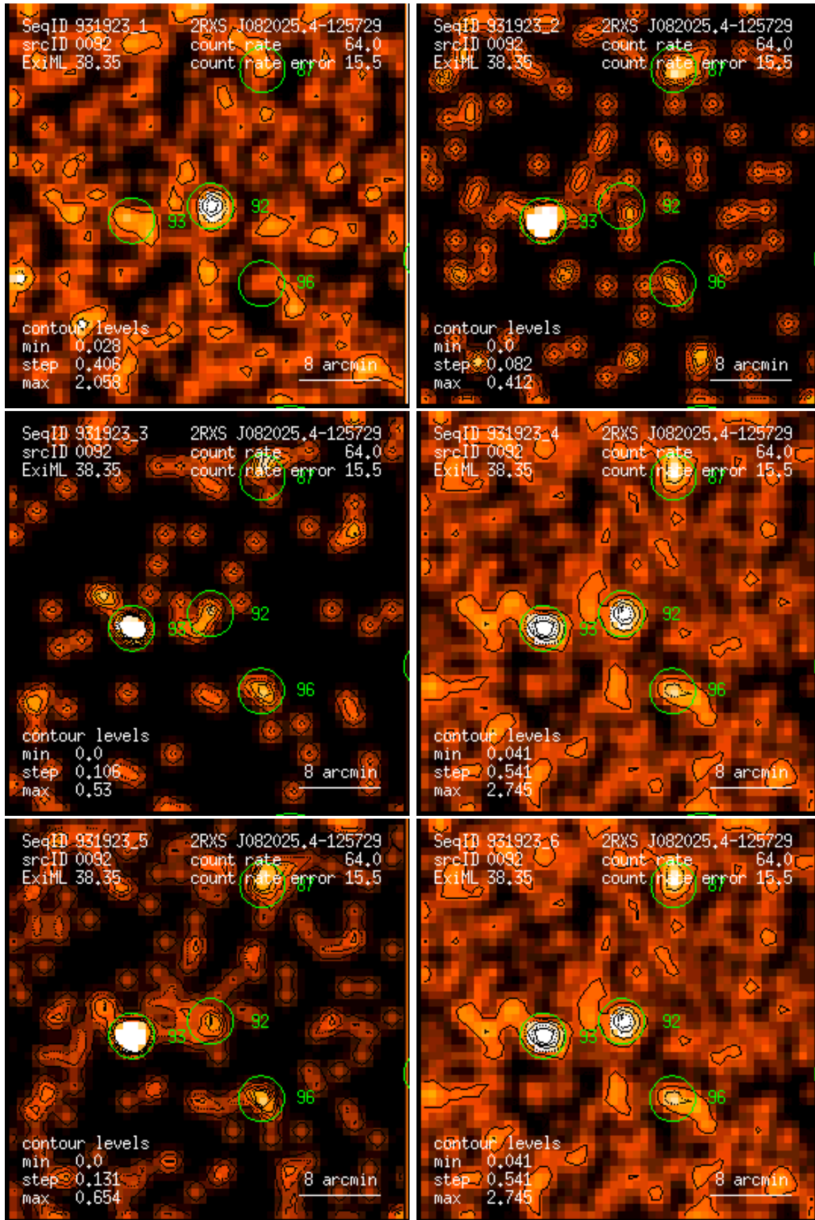
Figure 92: RASS 931923: detection 0092: band rate images, Gaussian filter: (1) PSPC channels 11 – 41, (2) 52 – 90, (3) 91 – 201, (4) 11 – 235, (5) 52 – 201, (6) 11 – 201. Broad band rates in counts/ks. Band rate contour levels in counts/ks/arcmin 2 .
