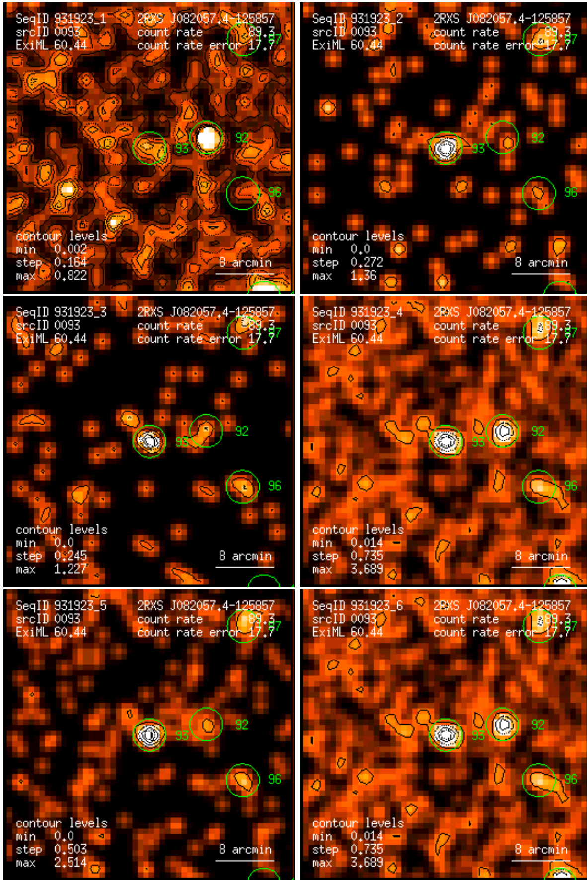
Figure 93: RASS 931923: detection 0093: band rate images, Gaussian filter: (1) PSPC channels 11 – 41, (2) 52 – 90, (3) 91 – 201, (4) 11 – 235, (5) 52 – 201, (6) 11 – 201. Broad band rates in counts/ks. Band rate contour levels in counts/ks/arcmin 2 .
