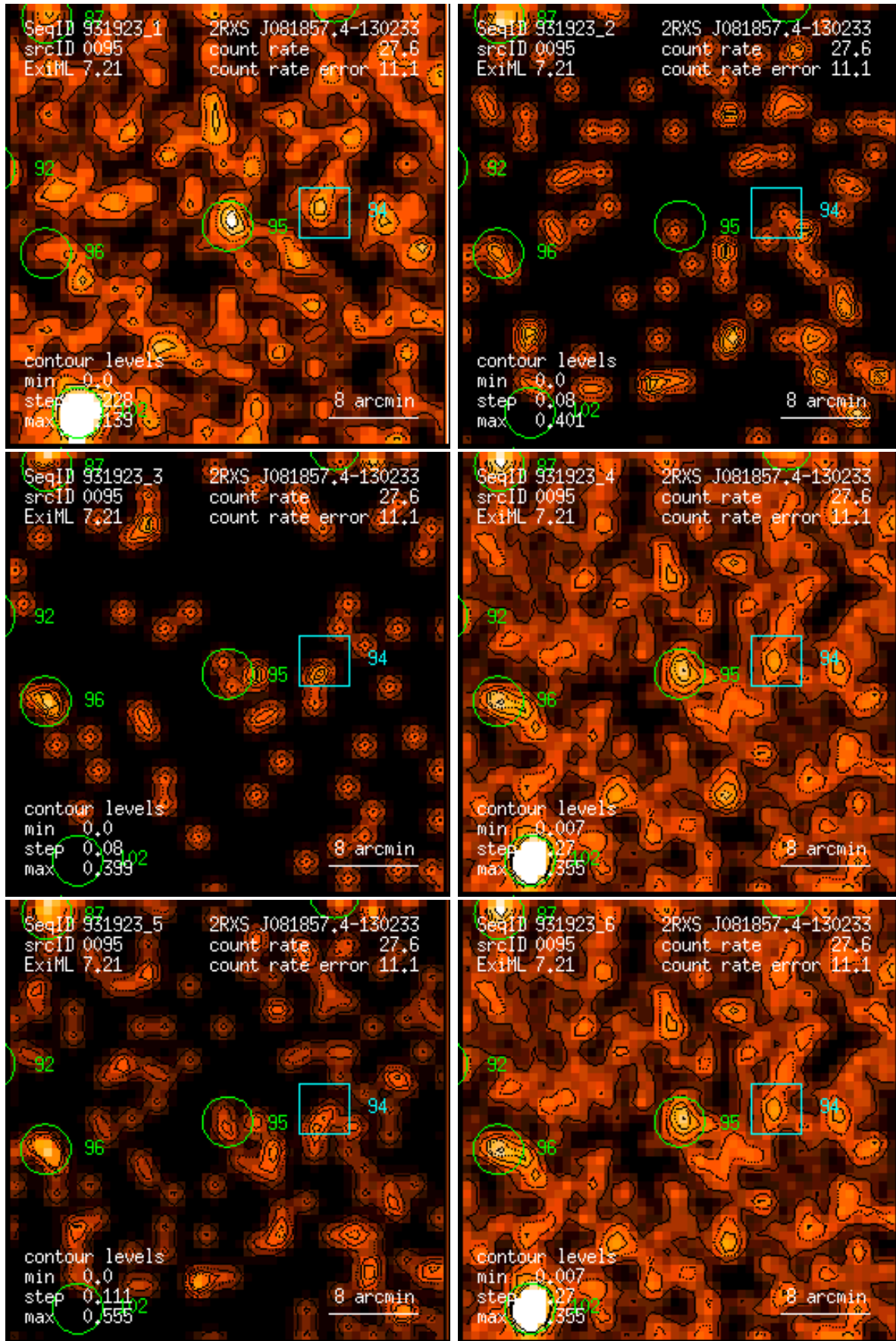
Figure 95: RASS 931923: detection 0095: band rate images, Gaussian filter: (1) PSPC channels 11 – 41, (2) 52 – 90, (3) 91 – 201, (4) 11 – 235, (5) 52 – 201, (6) 11 – 201. Broad band rates in counts/ks. Band rate contour levels in counts/ks/arcmin 2 .
