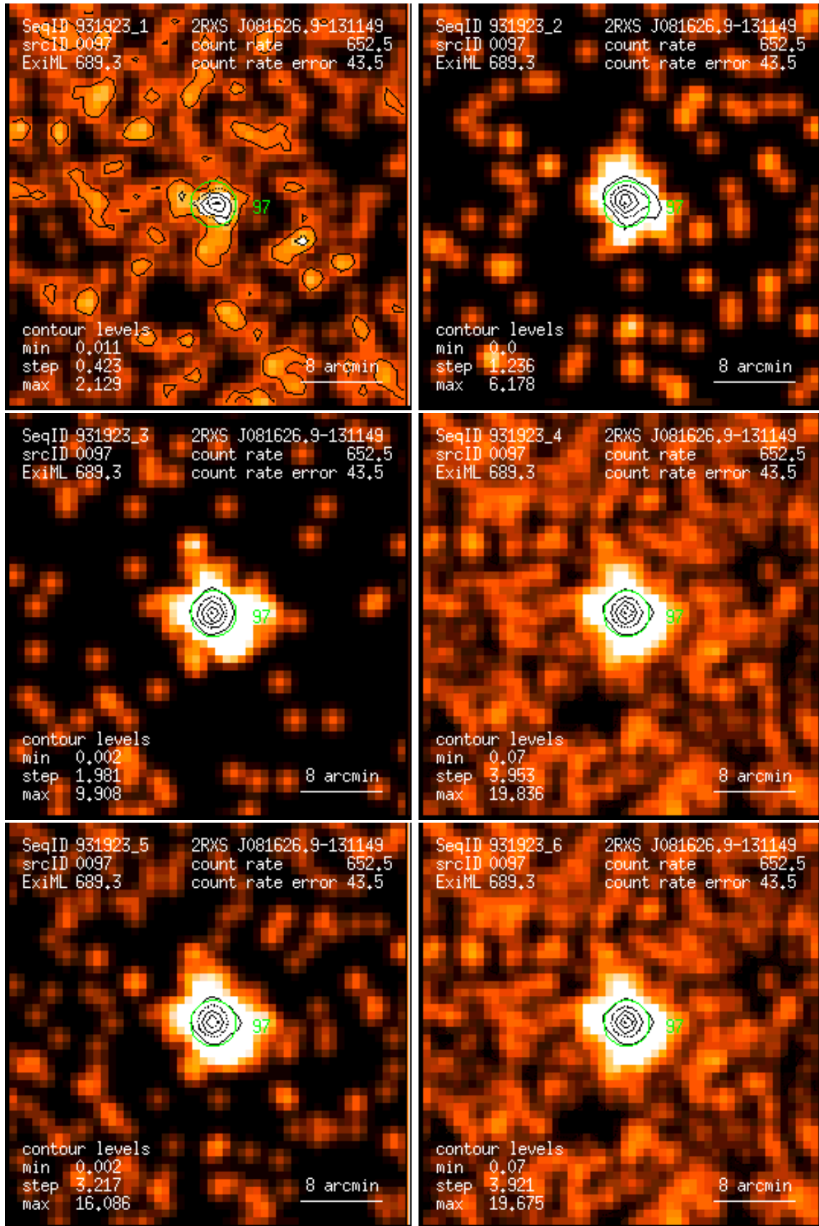
Figure 97: RASS 931923: detection 0097: band rate images, Gaussian filter: (1) PSPC channels 11 – 41, (2) 52 – 90, (3) 91 – 201, (4) 11 – 235, (5) 52 – 201, (6) 11 – 201. Broad band rates in counts/ks. Band rate contour levels in counts/ks/arcmin 2 .
