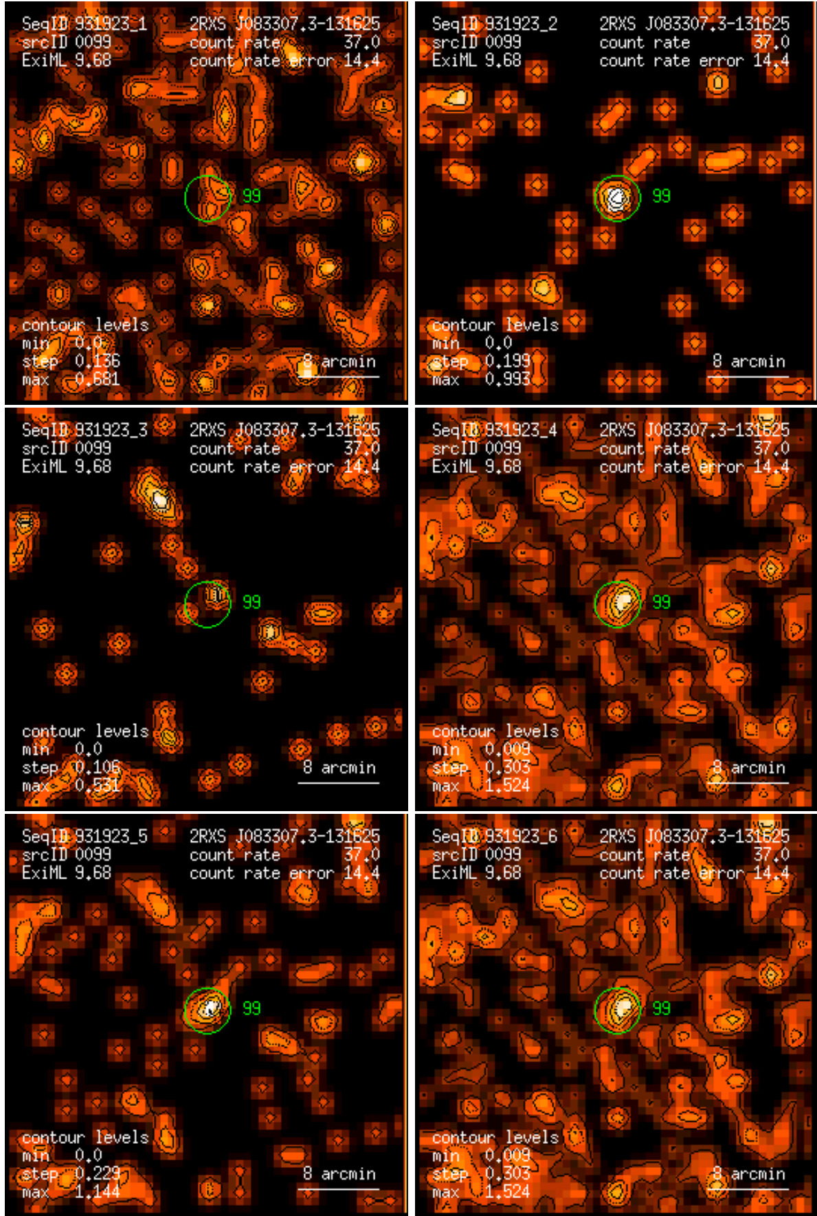
Figure 99: RASS 931923: detection 0099: band rate images, Gaussian filter: (1) PSPC channels 11 – 41, (2) 52 – 90, (3) 91 – 201, (4) 11 – 235, (5) 52 – 201, (6) 11 – 201. Broad band rates in counts/ks. Band rate contour levels in counts/ks/arcmin 2 .
