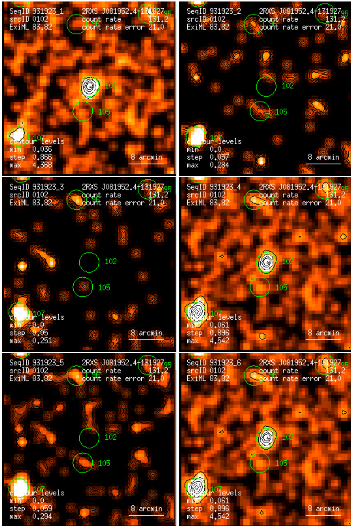
Figure 102: RASS 931923: detection 0102: band rate images, Gaussian filter: (1) PSPC channels 11 – 41, (2) 52 – 90, (3) 91 – 201, (4) 11 – 235, (5) 52 – 201, (6) 11 – 201. Broad band rates in counts/ks. Band rate contour levels in counts/ks/arcmin 2 .
