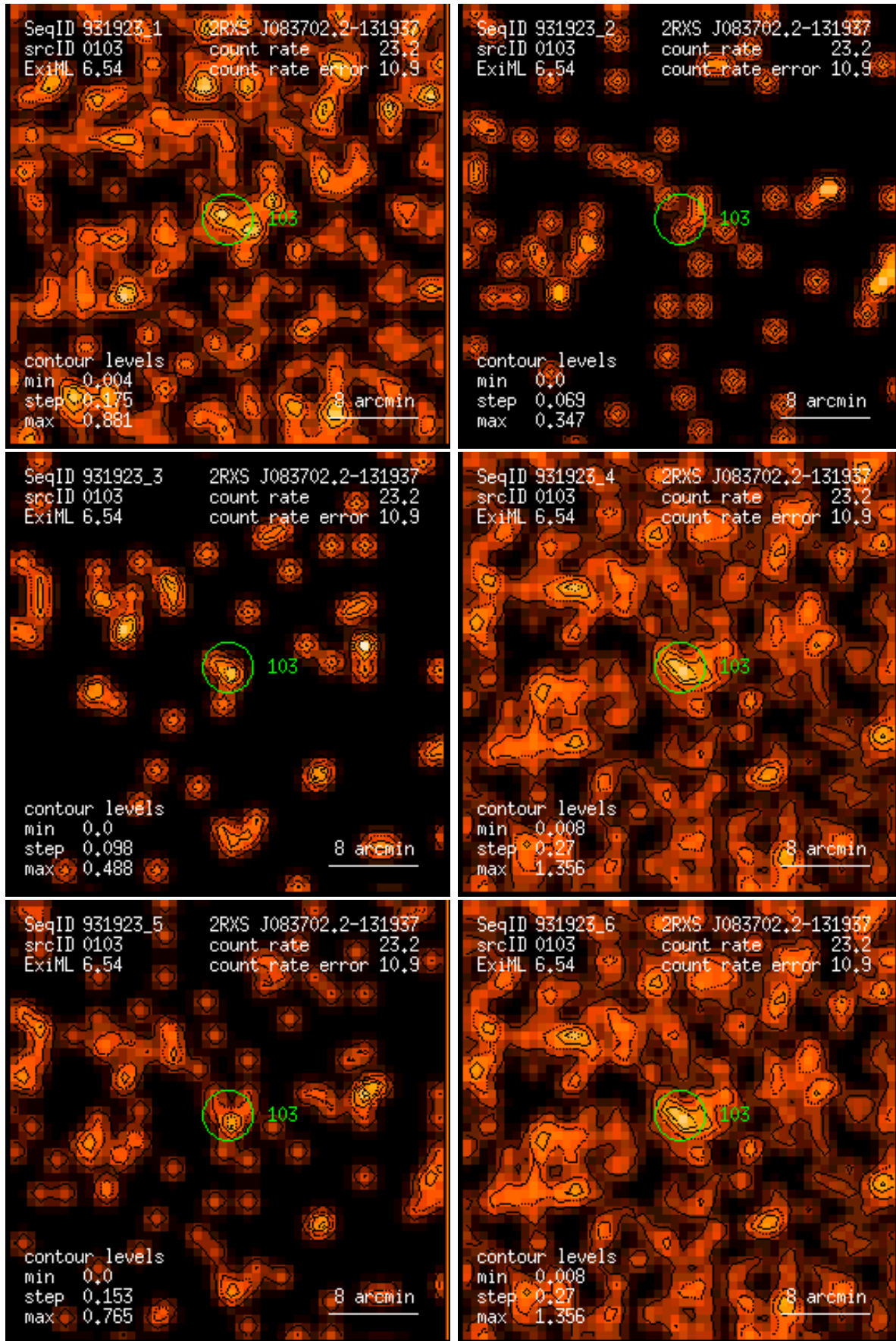
Figure 103: RASS 931923: detection 0103: band rate images, Gaussian filter: (1) PSPC channels 11 – 41, (2) 52 – 90, (3) 91 – 201, (4) 11 – 235, (5) 52 – 201, (6) 11 – 201. Broad band rates in counts/ks. Band rate contour levels in counts/ks/arcmin 2 .
