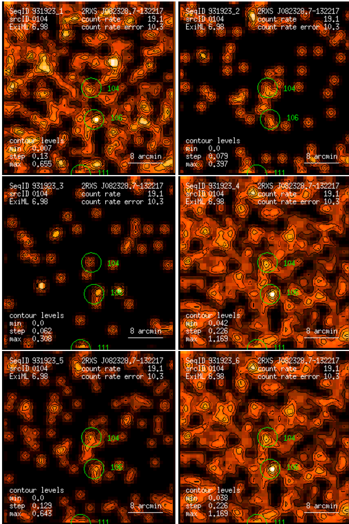
Figure 104: RASS 931923: detection 0104: band rate images, Gaussian filter: (1) PSPC channels 11 – 41, (2) 52 – 90, (3) 91 – 201, (4) 11 – 235, (5) 52 – 201, (6) 11 – 201. Broad band rates in counts/ks. Band rate contour levels in counts/ks/arcmin 2 .
