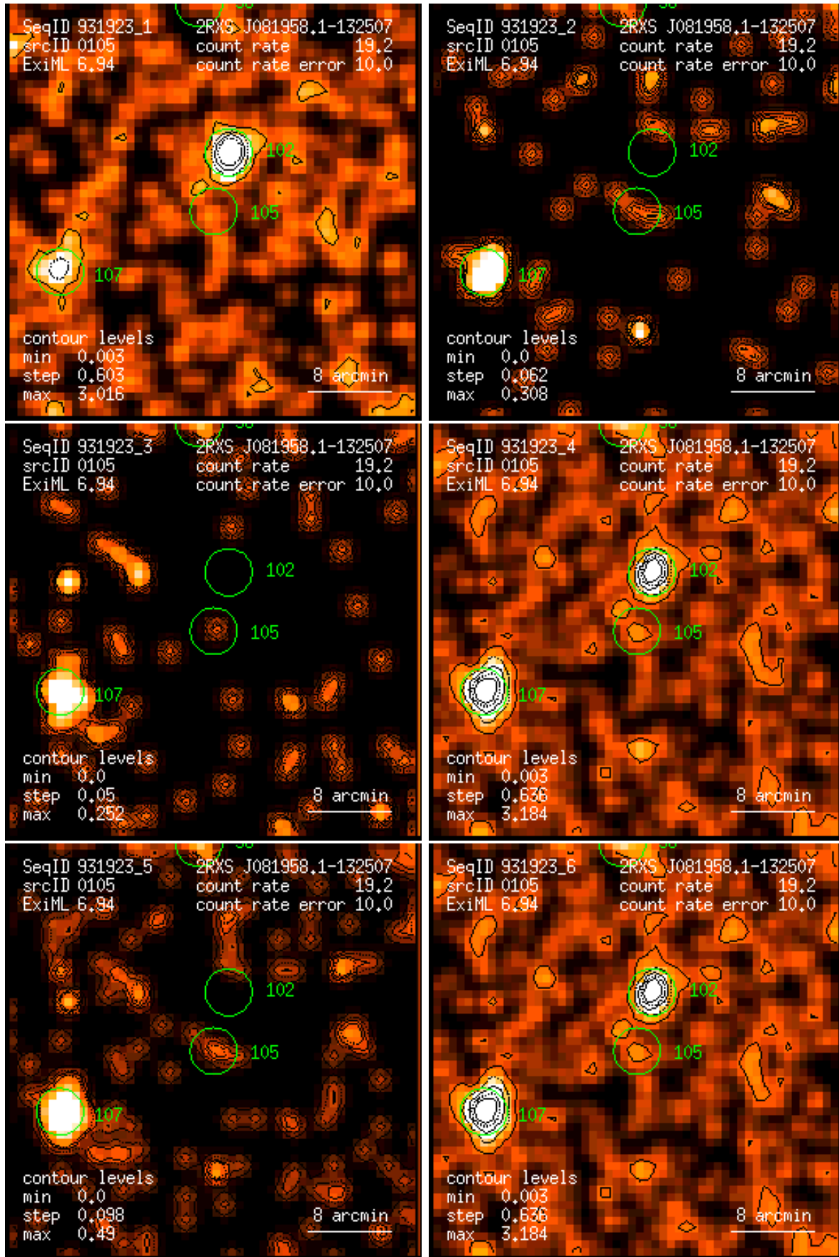
Figure 105: RASS 931923: detection 0105: band rate images, Gaussian filter: (1) PSPC channels 11 – 41, (2) 52 – 90, (3) 91 – 201, (4) 11 – 235, (5) 52 – 201, (6) 11 – 201. Broad band rates in counts/ks. Band rate contour levels in counts/ks/arcmin 2 .
