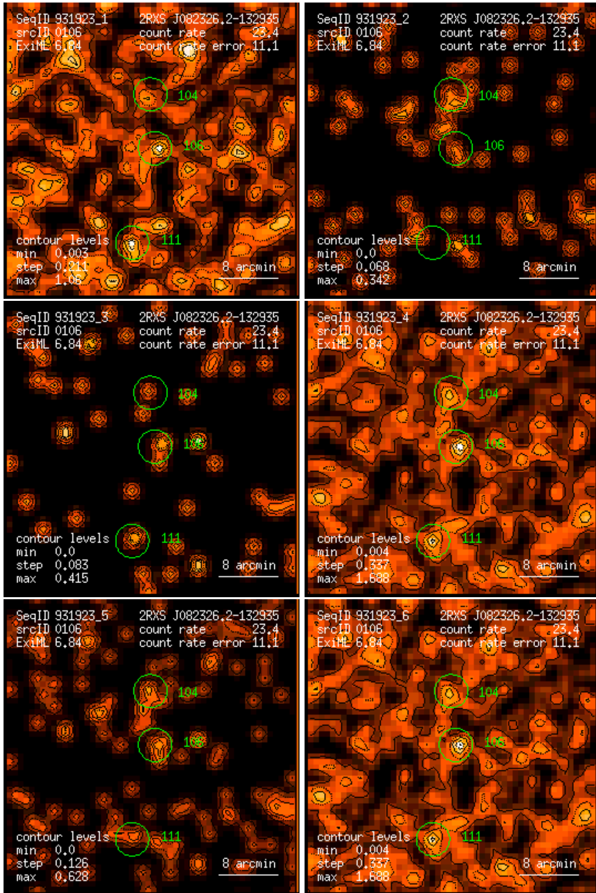
Figure 106: RASS 931923: detection 0106: band rate images, Gaussian filter: (1) PSPC channels 11 – 41, (2) 52 – 90, (3) 91 – 201, (4) 11 – 235, (5) 52 – 201, (6) 11 – 201. Broad band rates in counts/ks. Band rate contour levels in counts/ks/arcmin 2 .
