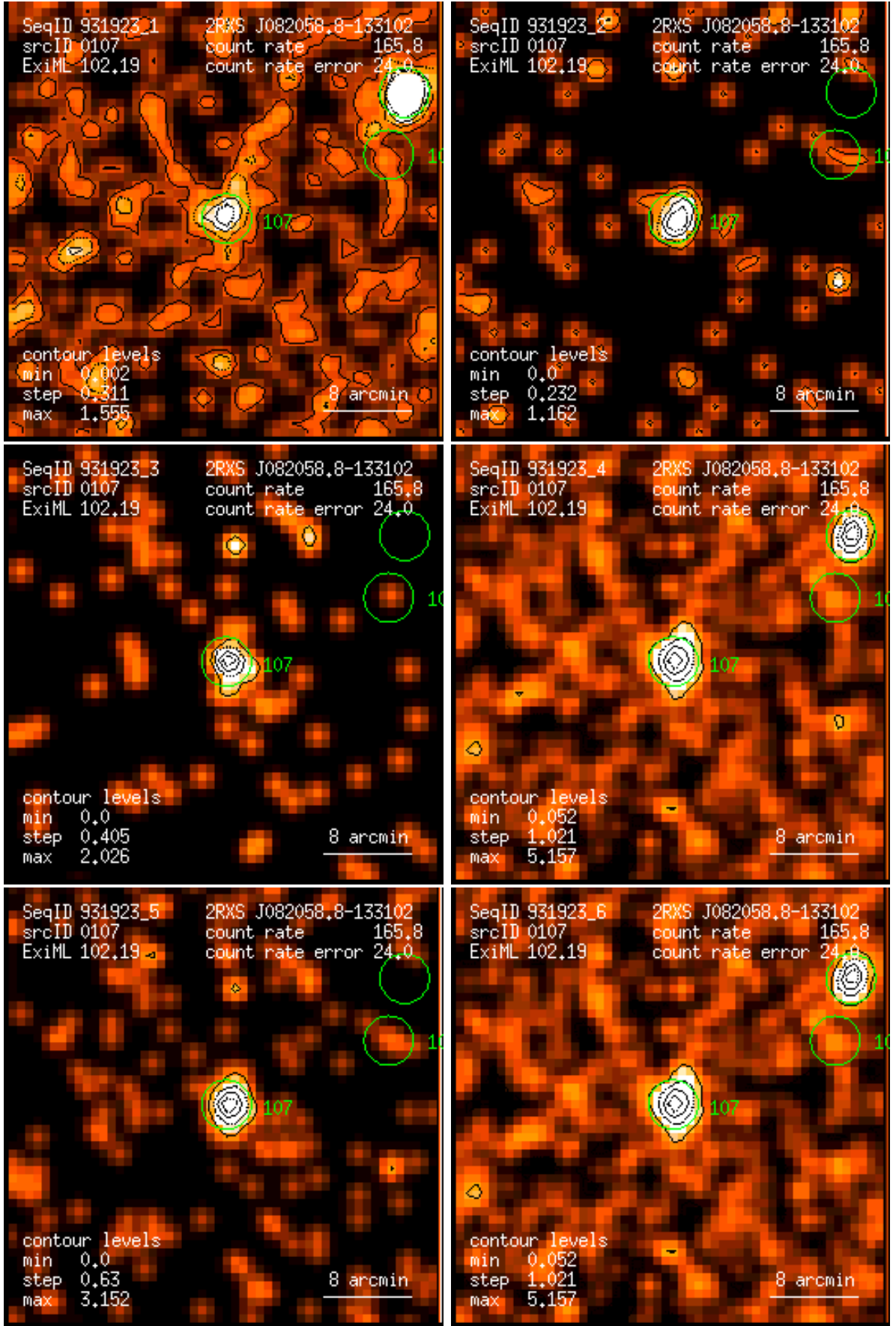
Figure 107: RASS 931923: detection 0107: band rate images, Gaussian filter: (1) PSPC channels 11 – 41, (2) 52 – 90, (3) 91 – 201, (4) 11 – 235, (5) 52 – 201, (6) 11 – 201. Broad band rates in counts/ks. Band rate contour levels in counts/ks/arcmin 2 .
