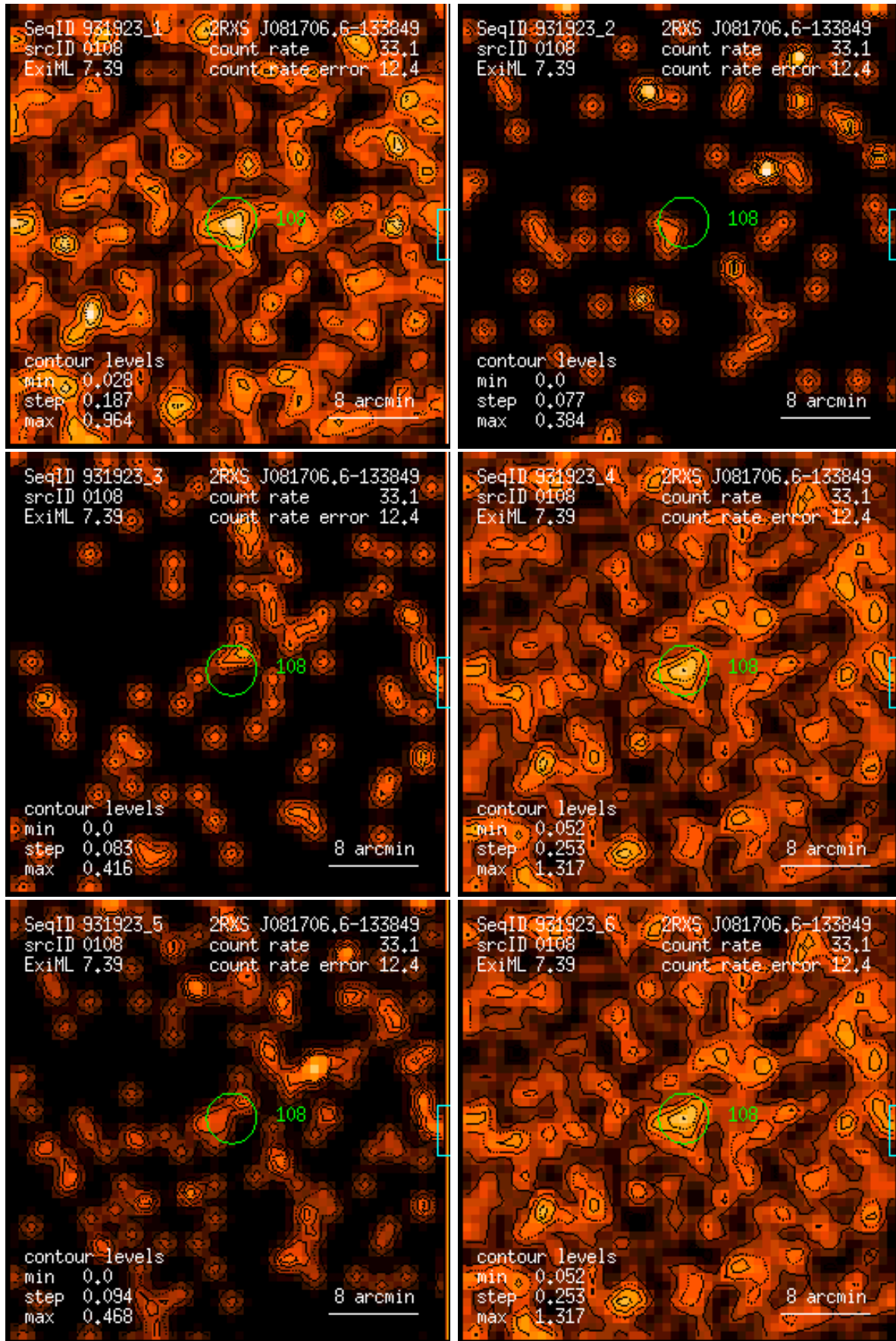
Figure 108: RASS 931923: detection 0108: band rate images, Gaussian filter: (1) PSPC channels 11 – 41, (2) 52 – 90, (3) 91 – 201, (4) 11 – 235, (5) 52 – 201, (6) 11 – 201. Broad band rates in counts/ks. Band rate contour levels in counts/ks/arcmin 2 .
