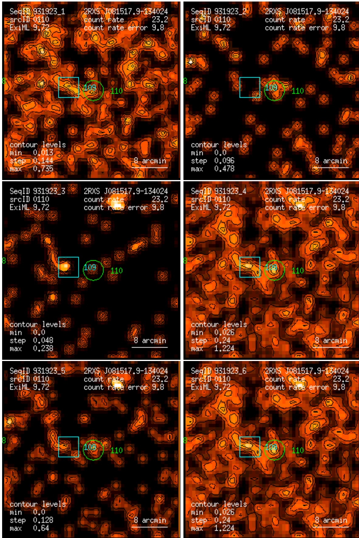
Figure 110: RASS 931923: detection 0110: band rate images, Gaussian filter: (1) PSPC channels 11 – 41, (2) 52 – 90, (3) 91 – 201, (4) 11 – 235, (5) 52 – 201, (6) 11 – 201. Broad band rates in counts/ks. Band rate contour levels in counts/ks/arcmin 2 .
