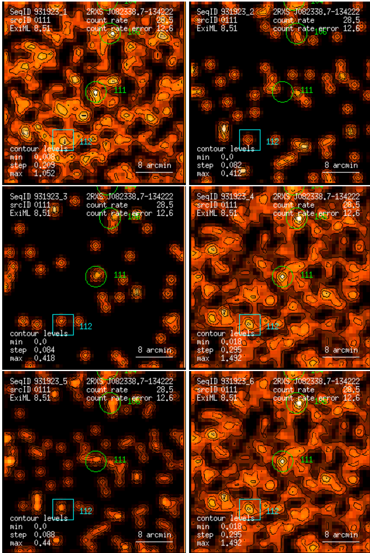
Figure 111: RASS 931923: detection 0111: band rate images, Gaussian filter: (1) PSPC channels 11 – 41, (2) 52 – 90, (3) 91 – 201, (4) 11 – 235, (5) 52 – 201, (6) 11 – 201. Broad band rates in counts/ks. Band rate contour levels in counts/ks/arcmin 2 .
