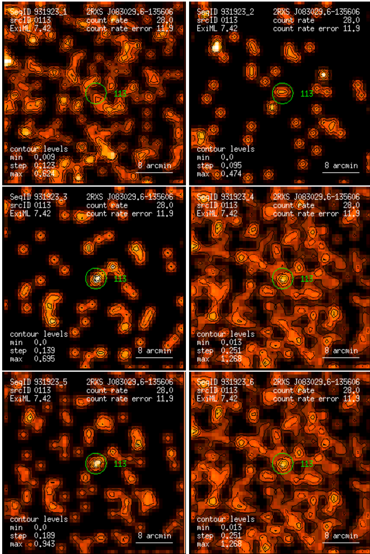
Figure 113: RASS 931923: detection 0113: band rate images, Gaussian filter: (1) PSPC channels 11 – 41, (2) 52 – 90, (3) 91 – 201, (4) 11 – 235, (5) 52 – 201, (6) 11 – 201. Broad band rates in counts/ks. Band rate contour levels in counts/ks/arcmin 2 .
