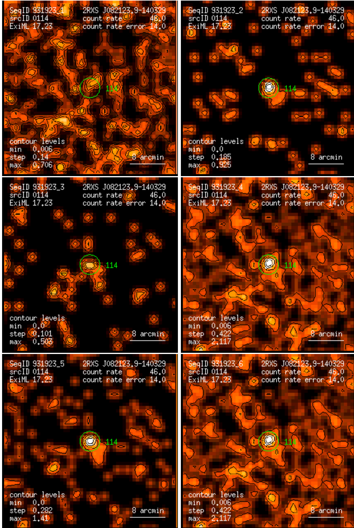
Figure 114: RASS 931923: detection 0114: band rate images, Gaussian filter: (1) PSPC channels 11 – 41, (2) 52 – 90, (3) 91 – 201, (4) 11 – 235, (5) 52 – 201, (6) 11 – 201. Broad band rates in counts/ks. Band rate contour levels in counts/ks/arcmin 2 .
