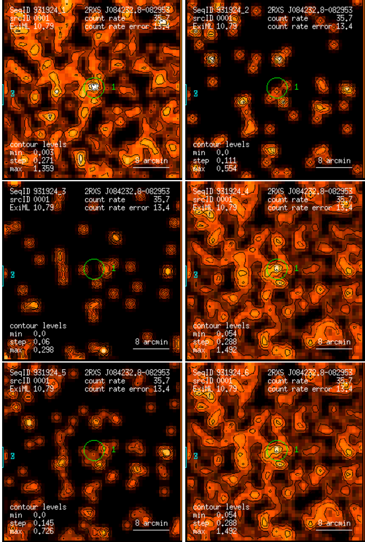
Figure 1: RASS 931924: detection 0001: band rate images, Gaussian filter: (1) PSPC channels 11 – 41, (2) 52 – 90, (3) 91 – 201, (4) 11 – 235, (5) 52 – 201, (6) 11 – 201. Broad band rates in counts/ks. Band rate contour levels in counts/ks/arcmin 2 .
