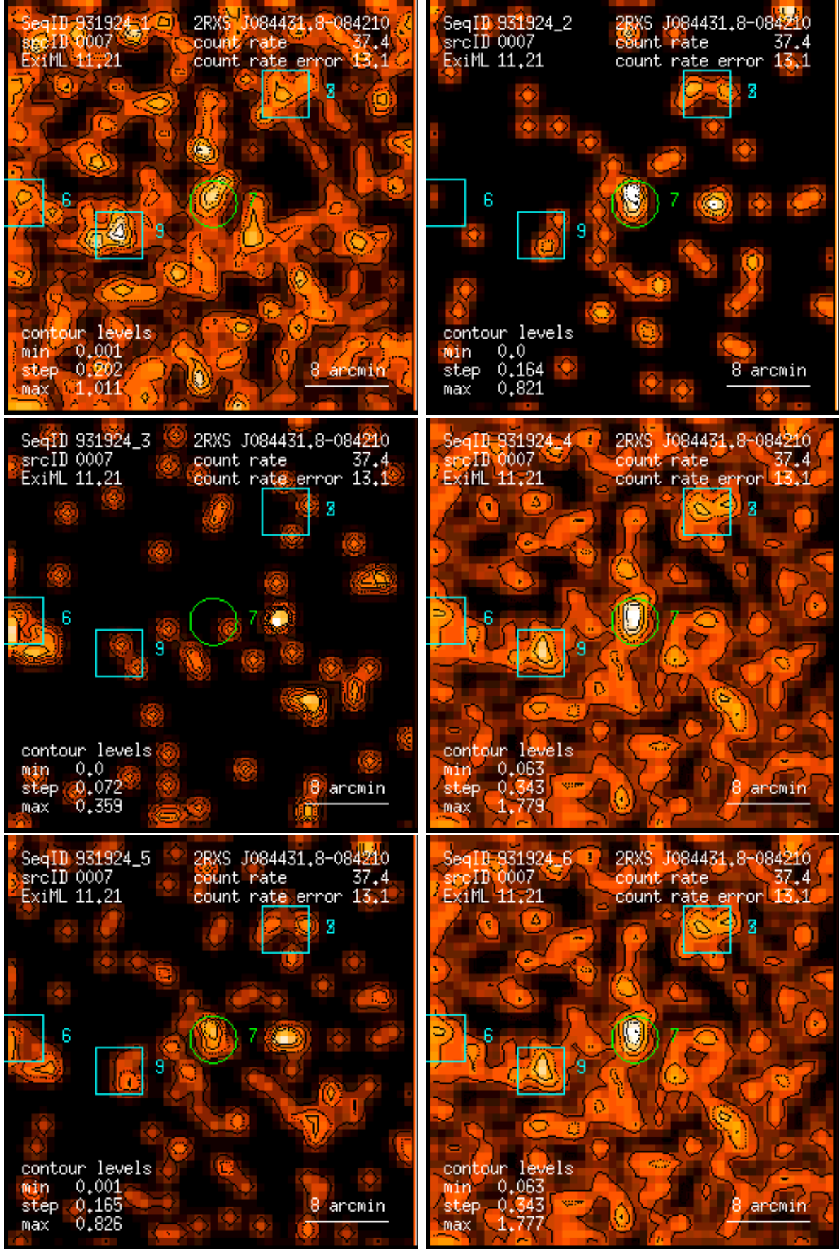
Figure 7: RASS 931924: detection 0007: band rate images, Gaussian filter: (1) PSPC channels 11 – 41, (2) 52 – 90, (3) 91 – 201, (4) 11 – 235, (5) 52 – 201, (6) 11 – 201. Broad band rates in counts/ks. Band rate contour levels in counts/ks/arcmin 2 .
