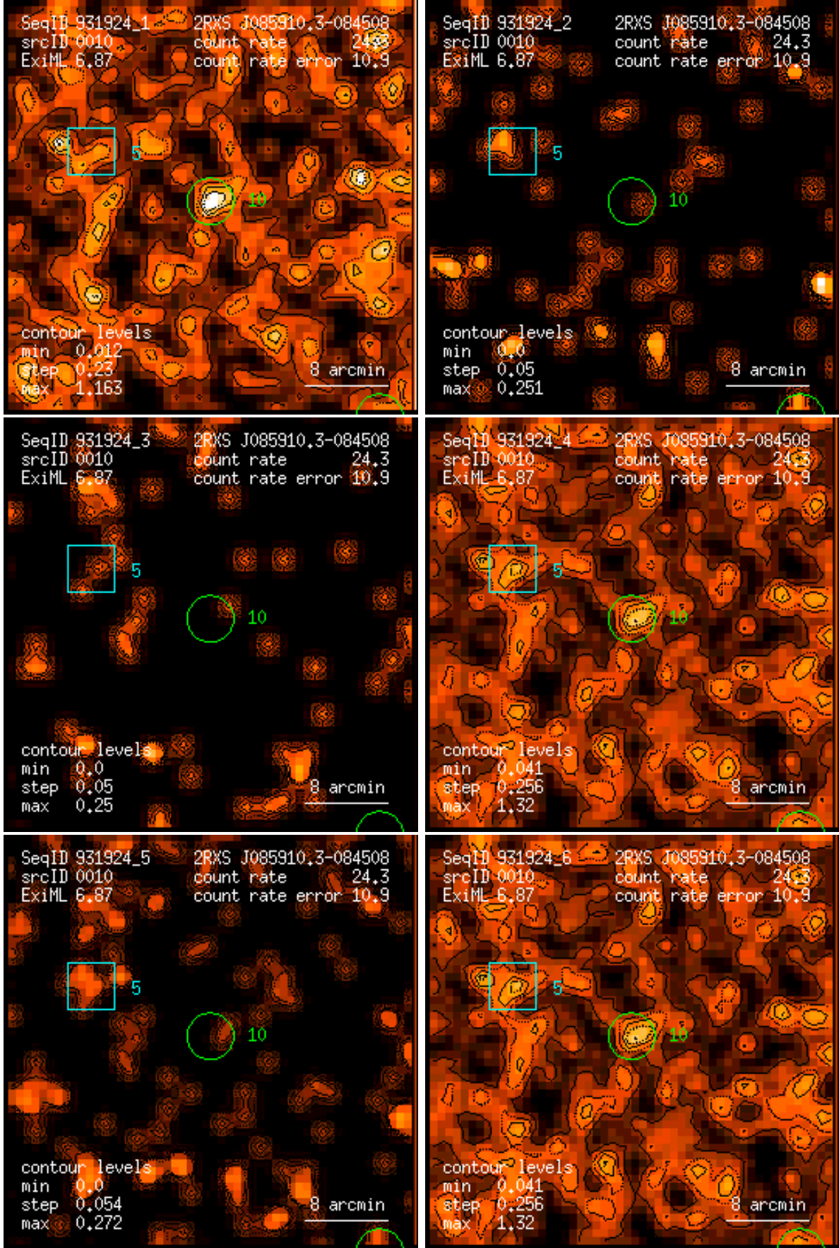
Figure 10: RASS 931924: detection 0010: band rate images, Gaussian filter: (1) PSPC channels 11 – 41, (2) 52 – 90, (3) 91 – 201, (4) 11 – 235, (5) 52 – 201, (6) 11 – 201. Broad band rates in counts/ks. Band rate contour levels in counts/ks/arcmin 2 .
