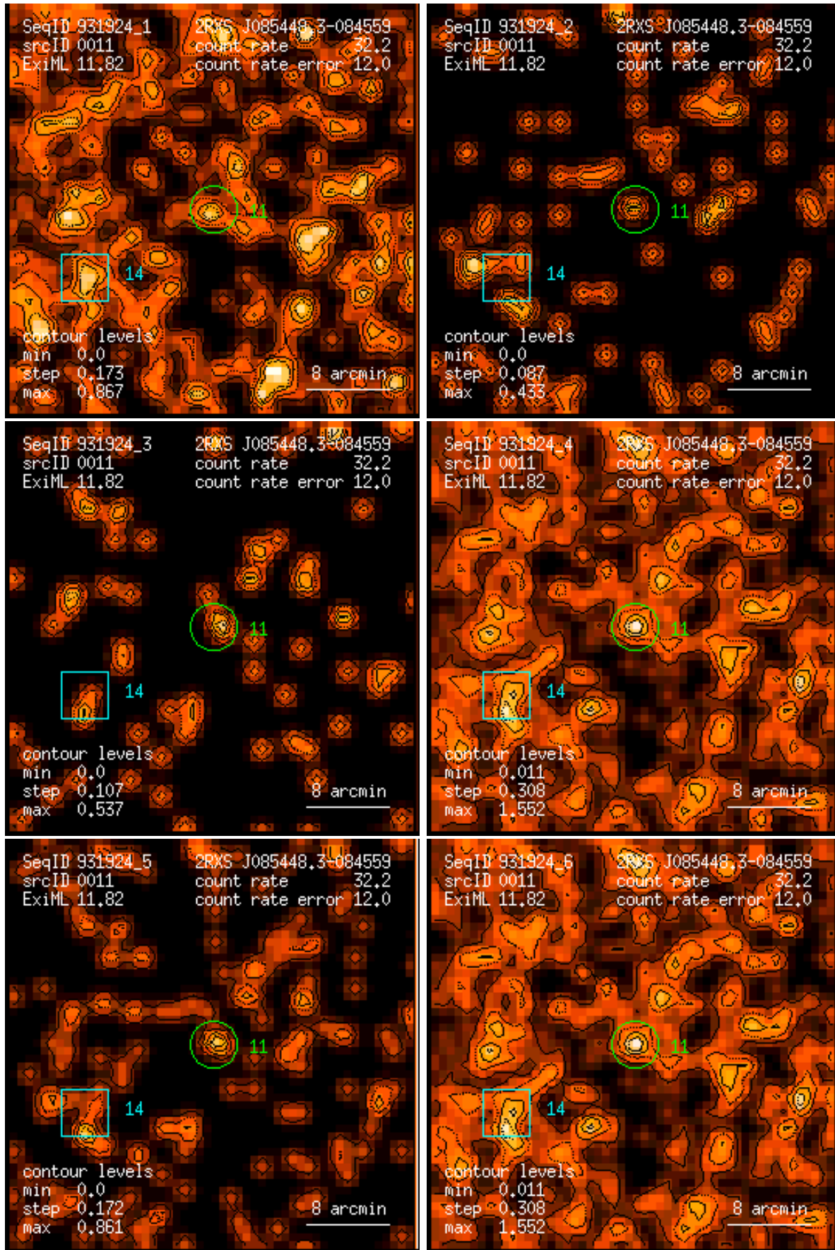
Figure 11: RASS 931924: detection 0011: band rate images, Gaussian filter: (1) PSPC channels 11 – 41, (2) 52 – 90, (3) 91 – 201, (4) 11 – 235, (5) 52 – 201, (6) 11 – 201. Broad band rates in counts/ks. Band rate contour levels in counts/ks/arcmin 2 .
