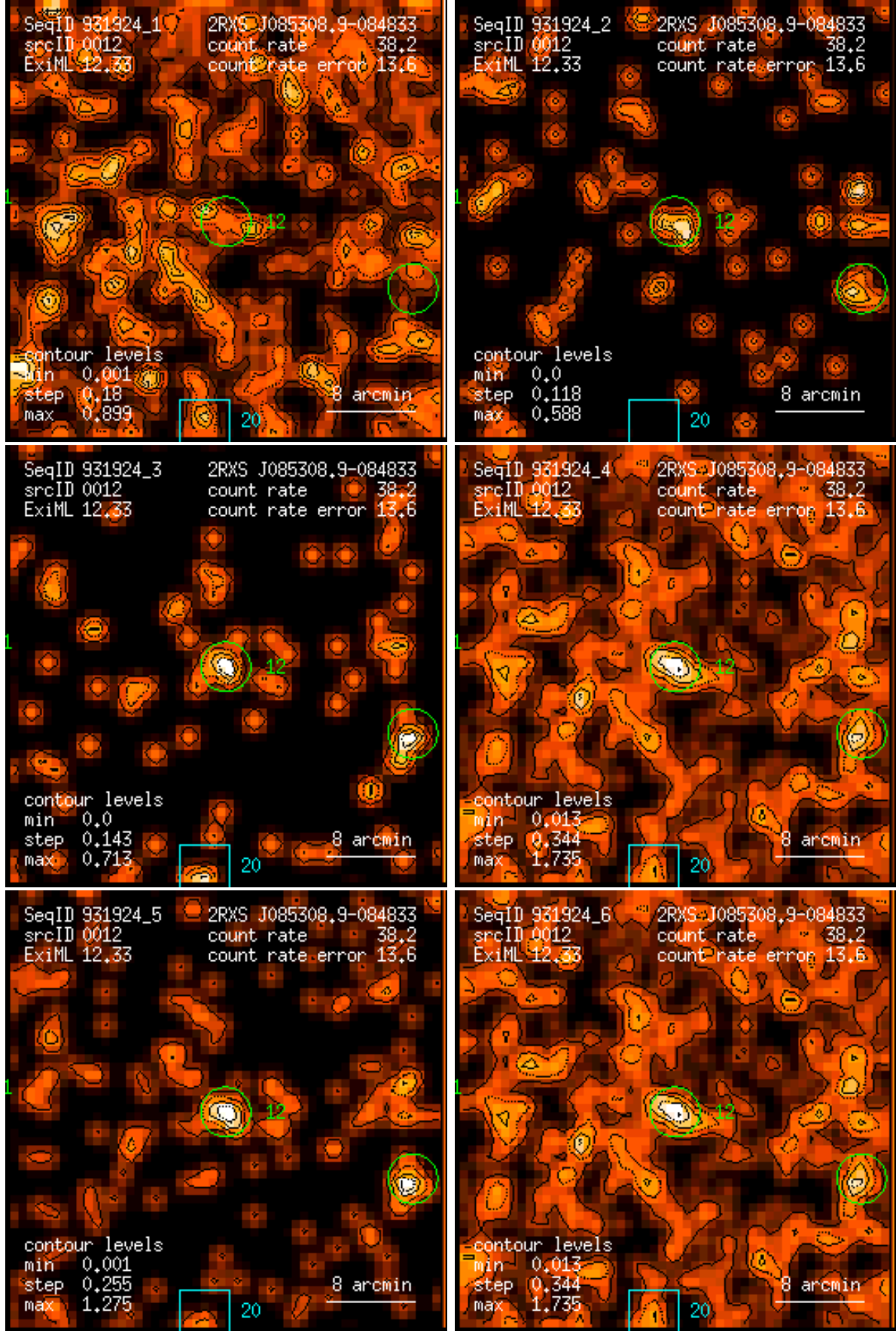
Figure 12: RASS 931924: detection 0012: band rate images, Gaussian filter: (1) PSPC channels 11 – 41, (2) 52 – 90, (3) 91 – 201, (4) 11 – 235, (5) 52 – 201, (6) 11 – 201. Broad band rates in counts/ks. Band rate contour levels in counts/ks/arcmin 2 .
