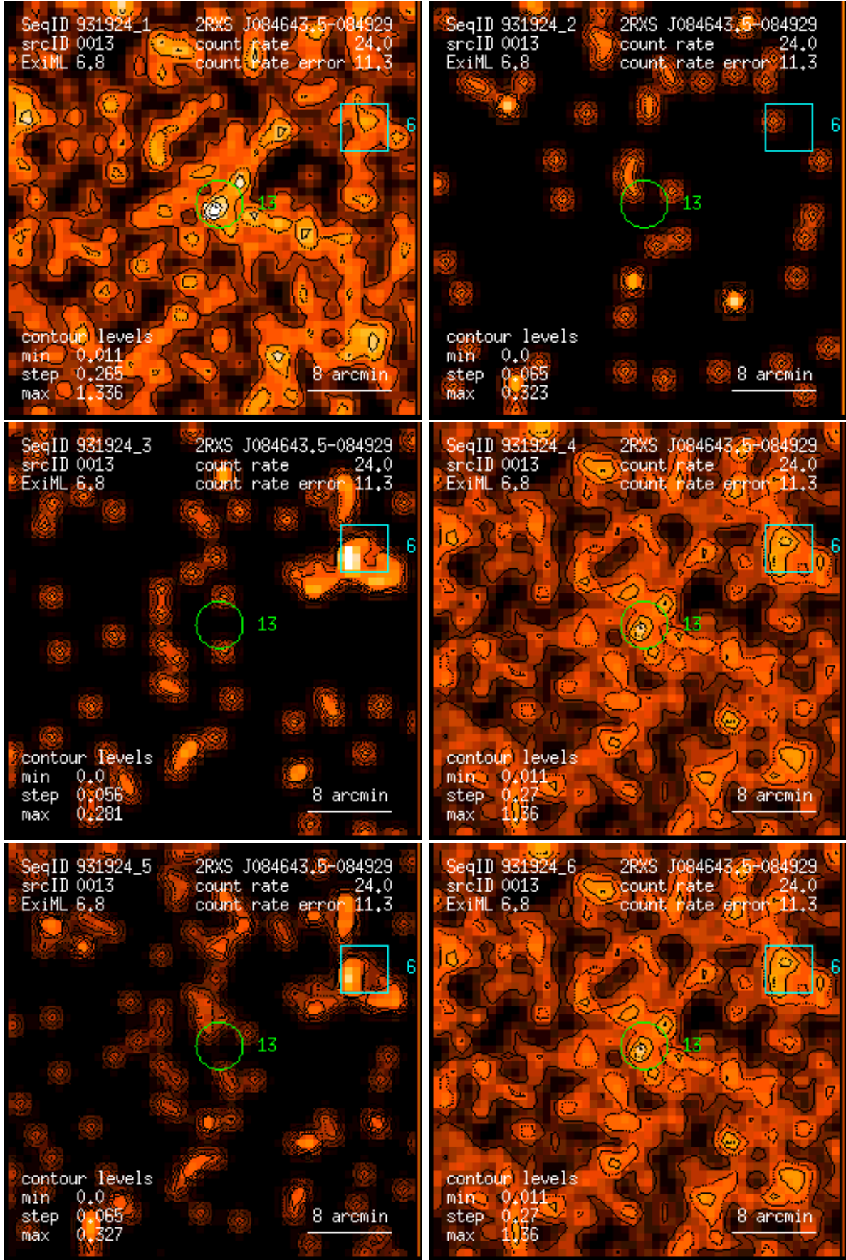
Figure 13: RASS 931924: detection 0013: band rate images, Gaussian filter: (1) PSPC channels 11 – 41, (2) 52 – 90, (3) 91 – 201, (4) 11 – 235, (5) 52 – 201, (6) 11 – 201. Broad band rates in counts/ks. Band rate contour levels in counts/ks/arcmin 2 .
