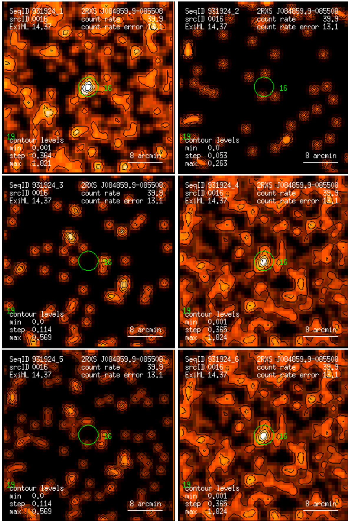
Figure 16: RASS 931924: detection 0016: band rate images, Gaussian filter: (1) PSPC channels 11 – 41, (2) 52 – 90, (3) 91 – 201, (4) 11 – 235, (5) 52 – 201, (6) 11 – 201. Broad band rates in counts/ks. Band rate contour levels in counts/ks/arcmin 2 .
