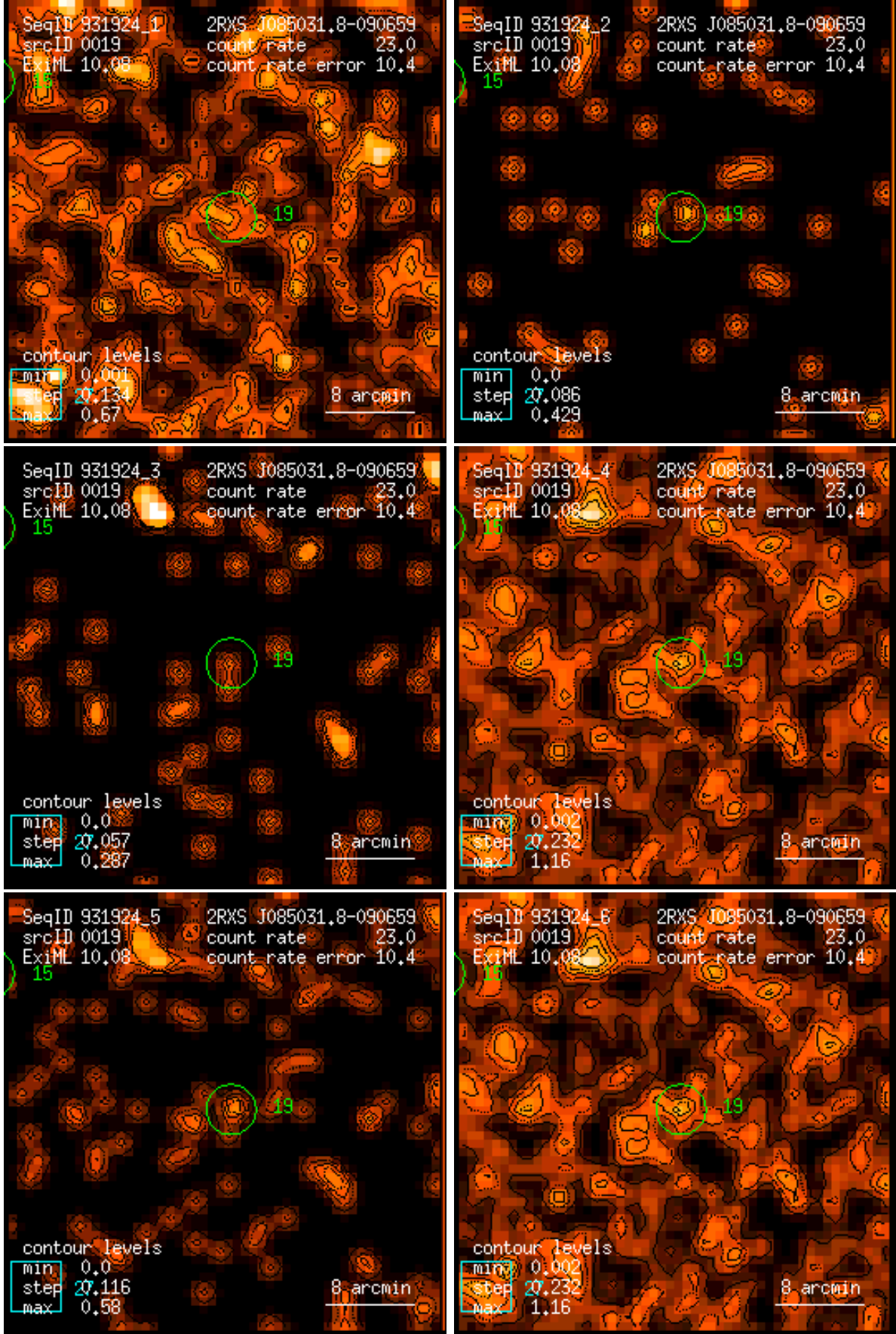
Figure 19: RASS 931924: detection 0019: band rate images, Gaussian filter: (1) PSPC channels 11 – 41, (2) 52 – 90, (3) 91 – 201, (4) 11 – 235, (5) 52 – 201, (6) 11 – 201. Broad band rates in counts/ks. Band rate contour levels in counts/ks/arcmin 2 .
