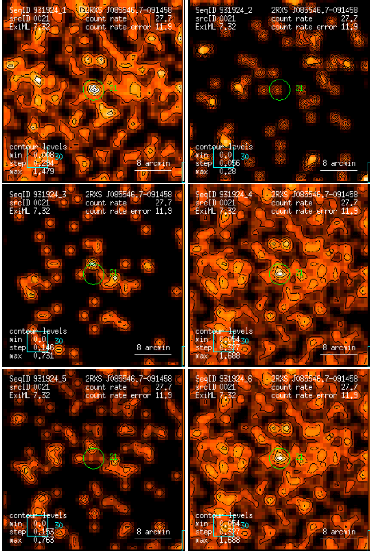
Figure 21: RASS 931924: detection 0021: band rate images, Gaussian filter: (1) PSPC channels 11 – 41, (2) 52 – 90, (3) 91 – 201, (4) 11 – 235, (5) 52 – 201, (6) 11 – 201. Broad band rates in counts/ks. Band rate contour levels in counts/ks/arcmin 2 .
