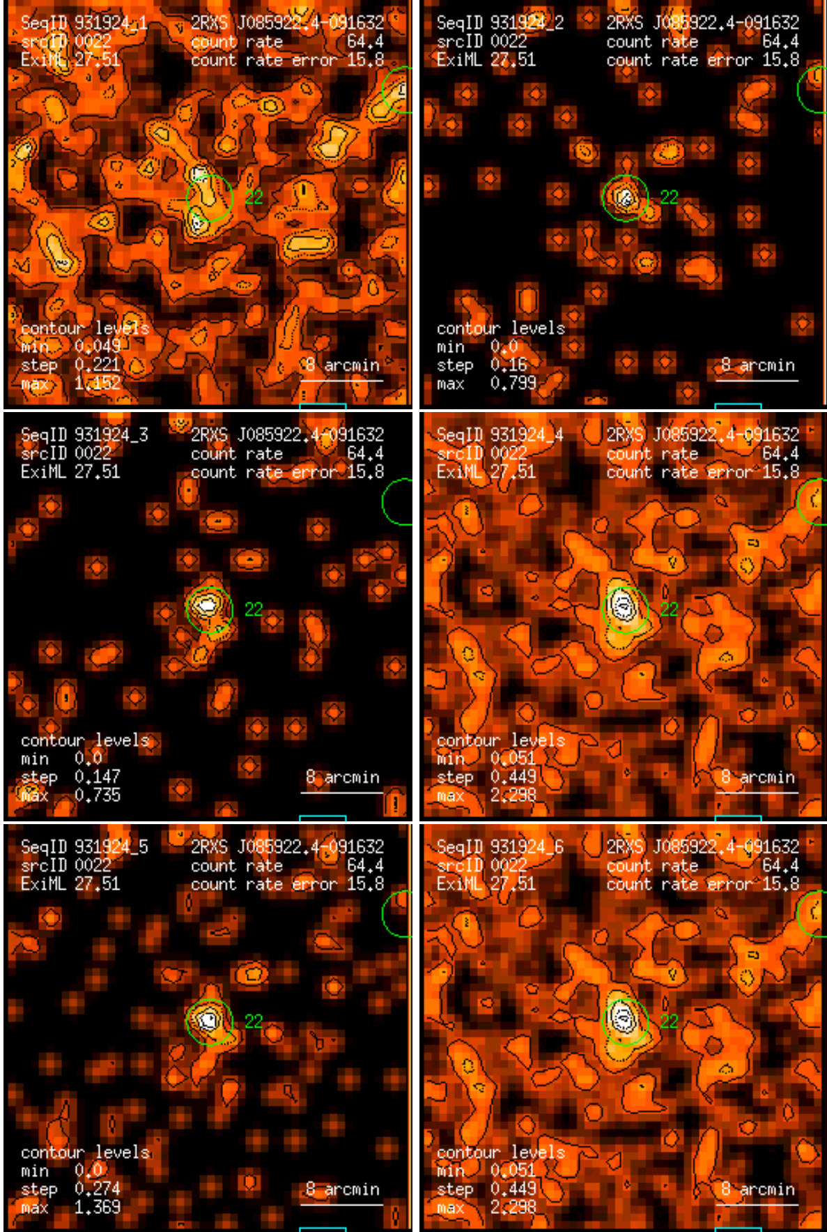
Figure 22: RASS 931924: detection 0022: band rate images, Gaussian filter: (1) PSPC channels 11 – 41, (2) 52 – 90, (3) 91 – 201, (4) 11 – 235, (5) 52 – 201, (6) 11 – 201. Broad band rates in counts/ks. Band rate contour levels in counts/ks/arcmin 2 .
