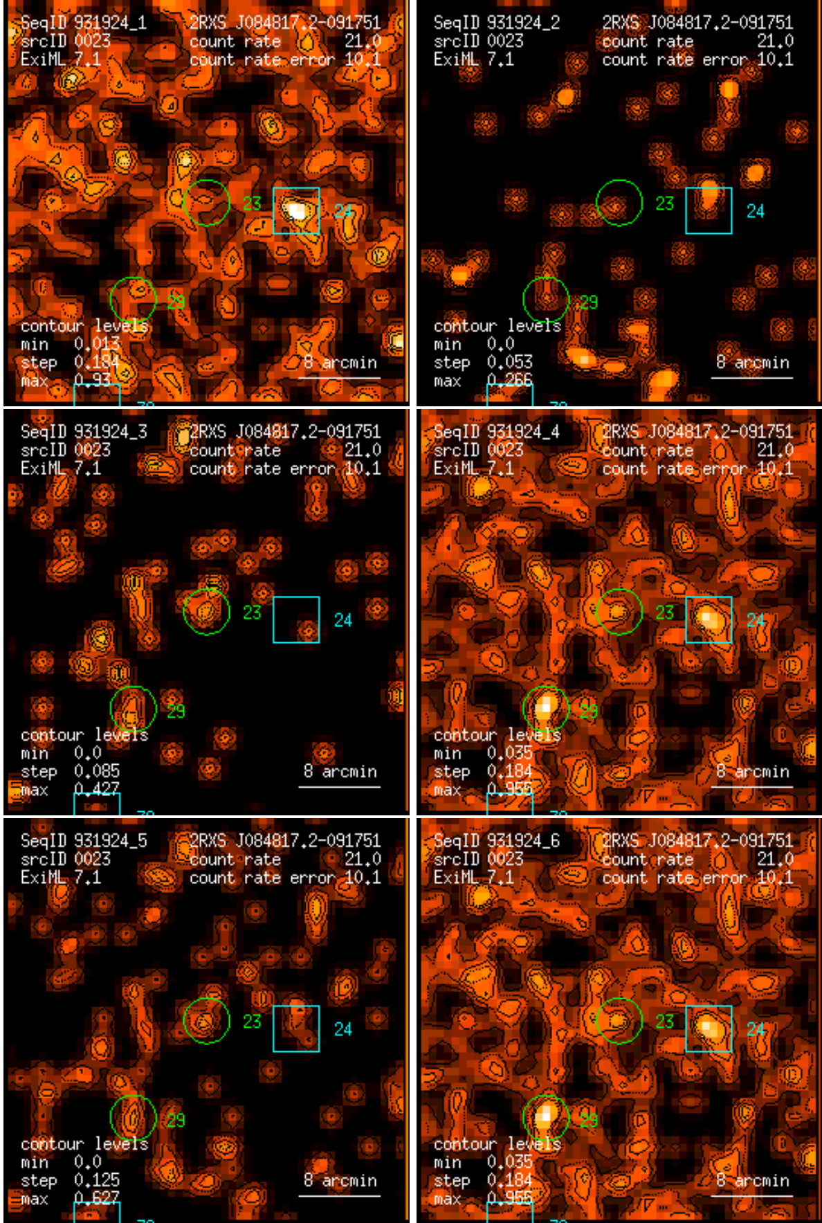
Figure 23: RASS 931924: detection 0023: band rate images, Gaussian filter: (1) PSPC channels 11 – 41, (2) 52 – 90, (3) 91 – 201, (4) 11 – 235, (5) 52 – 201, (6) 11 – 201. Broad band rates in counts/ks. Band rate contour levels in counts/ks/arcmin 2 .
