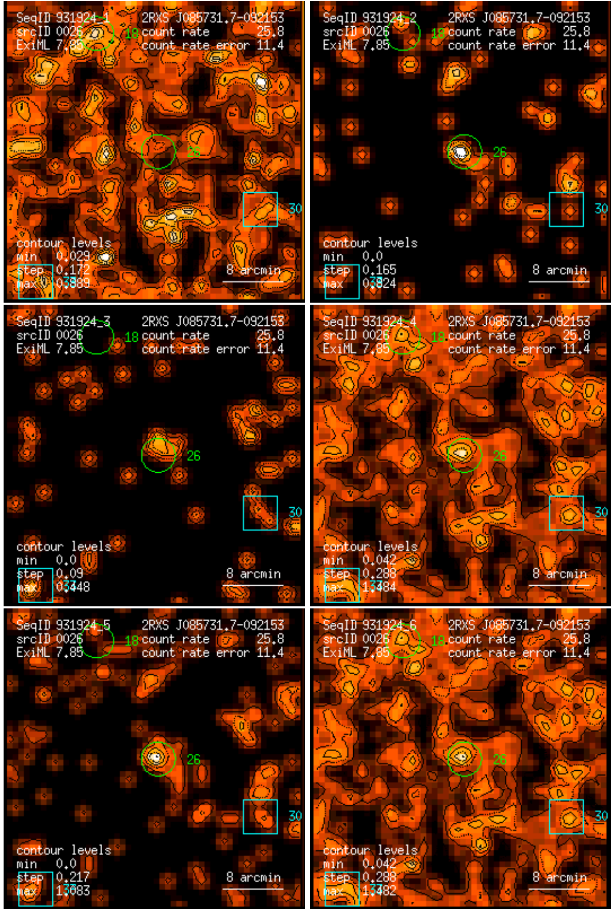
Figure 26: RASS 931924: detection 0026: band rate images, Gaussian filter: (1) PSPC channels 11 – 41, (2) 52 – 90, (3) 91 – 201, (4) 11 – 235, (5) 52 – 201, (6) 11 – 201. Broad band rates in counts/ks. Band rate contour levels in counts/ks/arcmin 2 .
