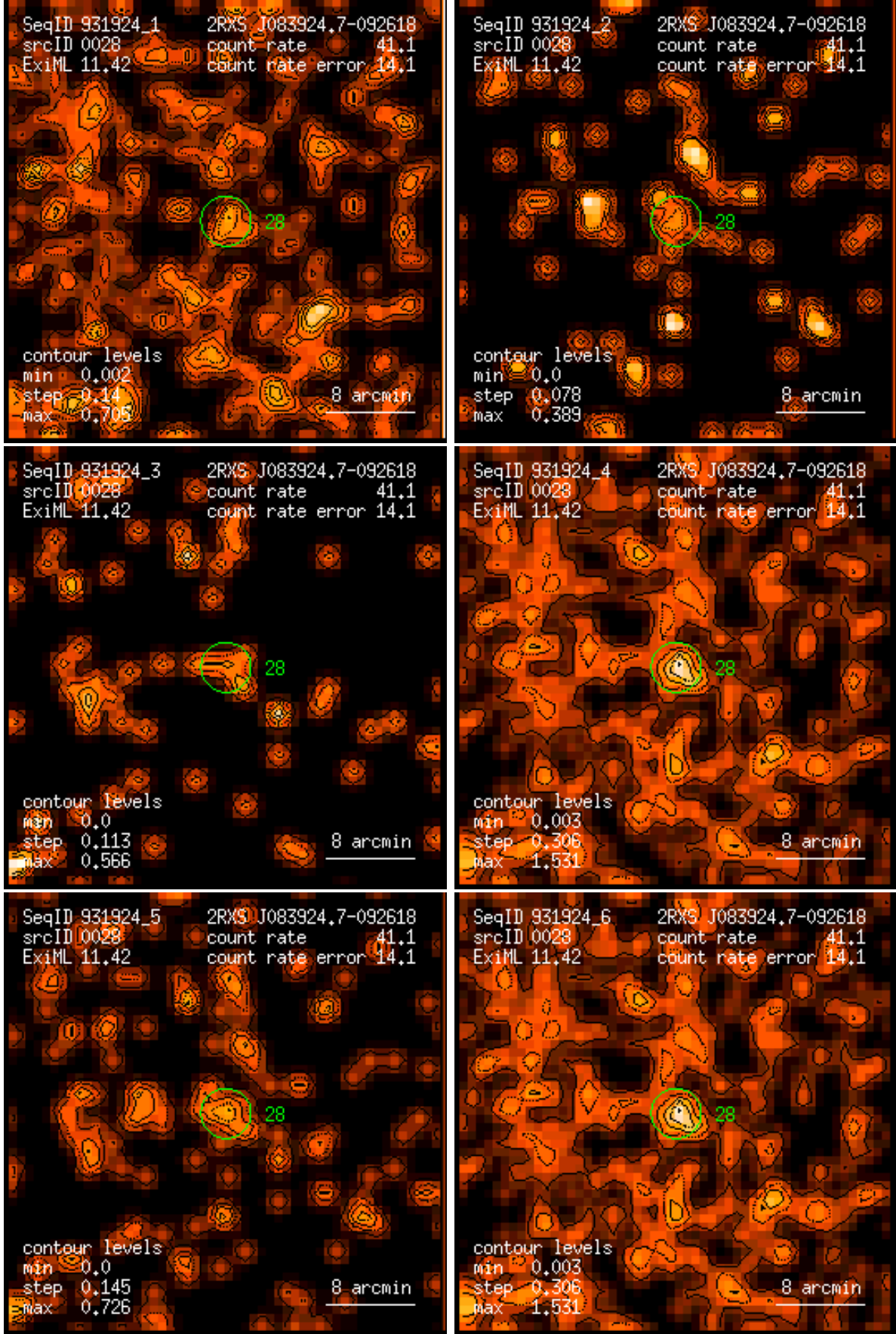
Figure 28: RASS 931924: detection 0028: band rate images, Gaussian filter: (1) PSPC channels 11 – 41, (2) 52 – 90, (3) 91 – 201, (4) 11 – 235, (5) 52 – 201, (6) 11 – 201. Broad band rates in counts/ks. Band rate contour levels in counts/ks/arcmin 2 .
