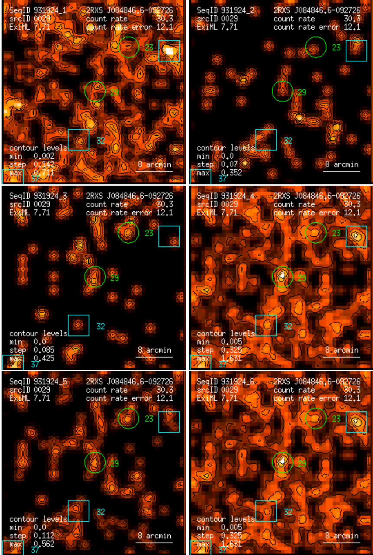
Figure 29: RASS 931924: detection 0029: band rate images, Gaussian filter: (1) PSPC channels 11 – 41, (2) 52 – 90, (3) 91 – 201, (4) 11 – 235, (5) 52 – 201, (6) 11 – 201. Broad band rates in counts/ks. Band rate contour levels in counts/ks/arcmin 2 .
