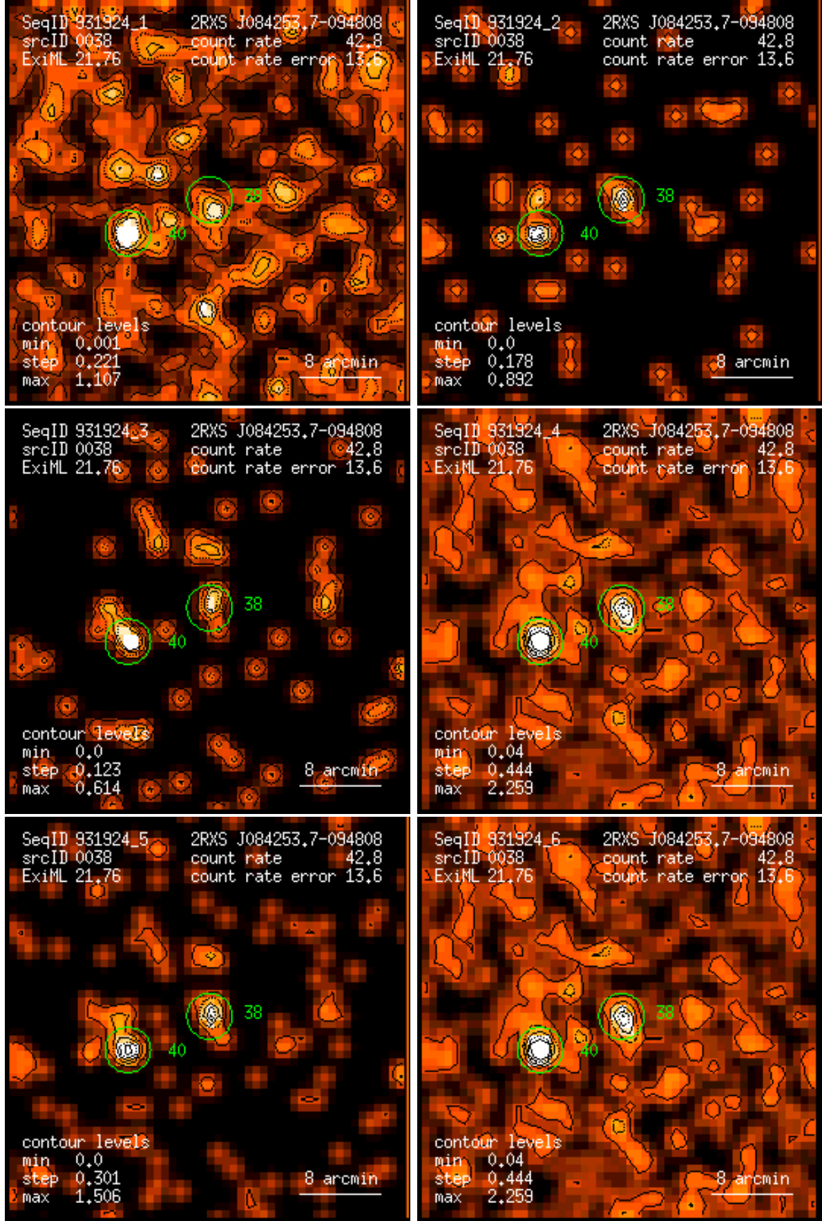
Figure 38: RASS 931924: detection 0038: band rate images, Gaussian filter: (1) PSPC channels 11 – 41, (2) 52 – 90, (3) 91 – 201, (4) 11 – 235, (5) 52 – 201, (6) 11 – 201. Broad band rates in counts/ks. Band rate contour levels in counts/ks/arcmin 2 .
