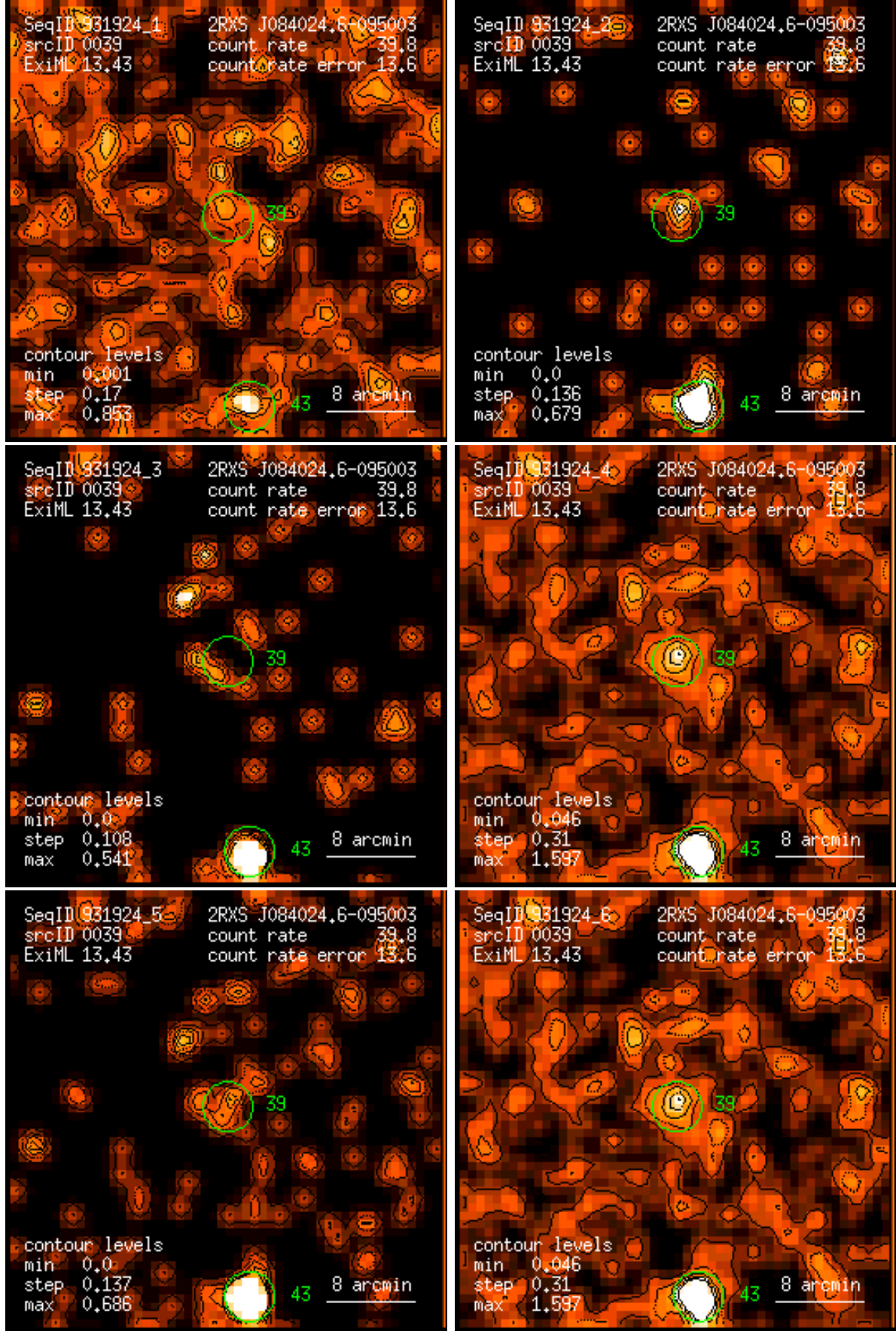
Figure 39: RASS 931924: detection 0039: band rate images, Gaussian filter: (1) PSPC channels 11 – 41, (2) 52 – 90, (3) 91 – 201, (4) 11 – 235, (5) 52 – 201, (6) 11 – 201. Broad band rates in counts/ks. Band rate contour levels in counts/ks/arcmin 2 .
