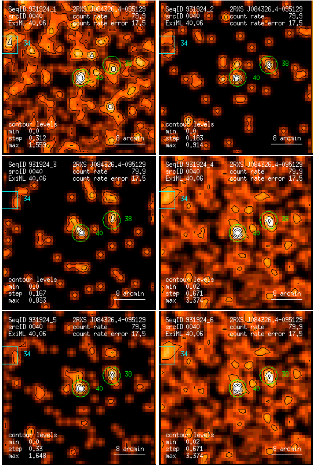
Figure 40: RASS 931924: detection 0040: band rate images, Gaussian filter: (1) PSPC channels 11 – 41, (2) 52 – 90, (3) 91 – 201, (4) 11 – 235, (5) 52 – 201, (6) 11 – 201. Broad band rates in counts/ks. Band rate contour levels in counts/ks/arcmin 2 .
