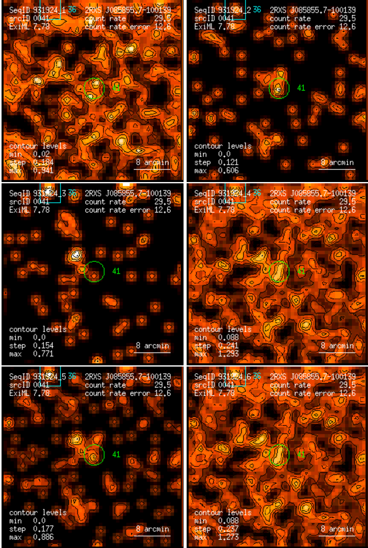
Figure 41: RASS 931924: detection 0041: band rate images, Gaussian filter: (1) PSPC channels 11 – 41, (2) 52 – 90, (3) 91 – 201, (4) 11 – 235, (5) 52 – 201, (6) 11 – 201. Broad band rates in counts/ks. Band rate contour levels in counts/ks/arcmin 2 .
