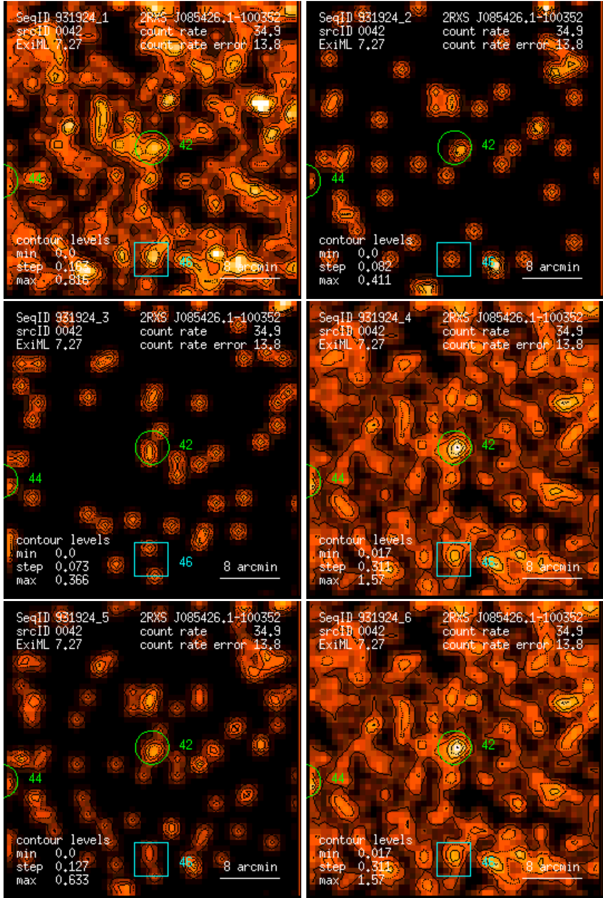
Figure 42: RASS 931924: detection 0042: band rate images, Gaussian filter: (1) PSPC channels 11 – 41, (2) 52 – 90, (3) 91 – 201, (4) 11 – 235, (5) 52 – 201, (6) 11 – 201. Broad band rates in counts/ks. Band rate contour levels in counts/ks/arcmin 2 .
