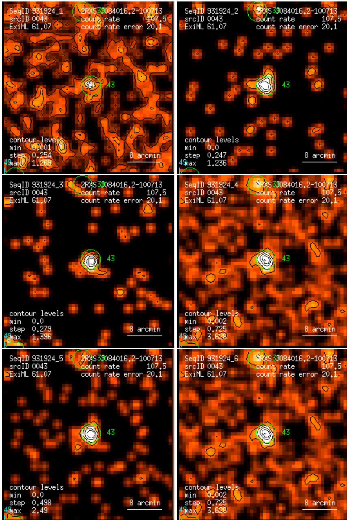
Figure 43: RASS 931924: detection 0043: band rate images, Gaussian filter: (1) PSPC channels 11 – 41, (2) 52 – 90, (3) 91 – 201, (4) 11 – 235, (5) 52 – 201, (6) 11 – 201. Broad band rates in counts/ks. Band rate contour levels in counts/ks/arcmin 2 .
