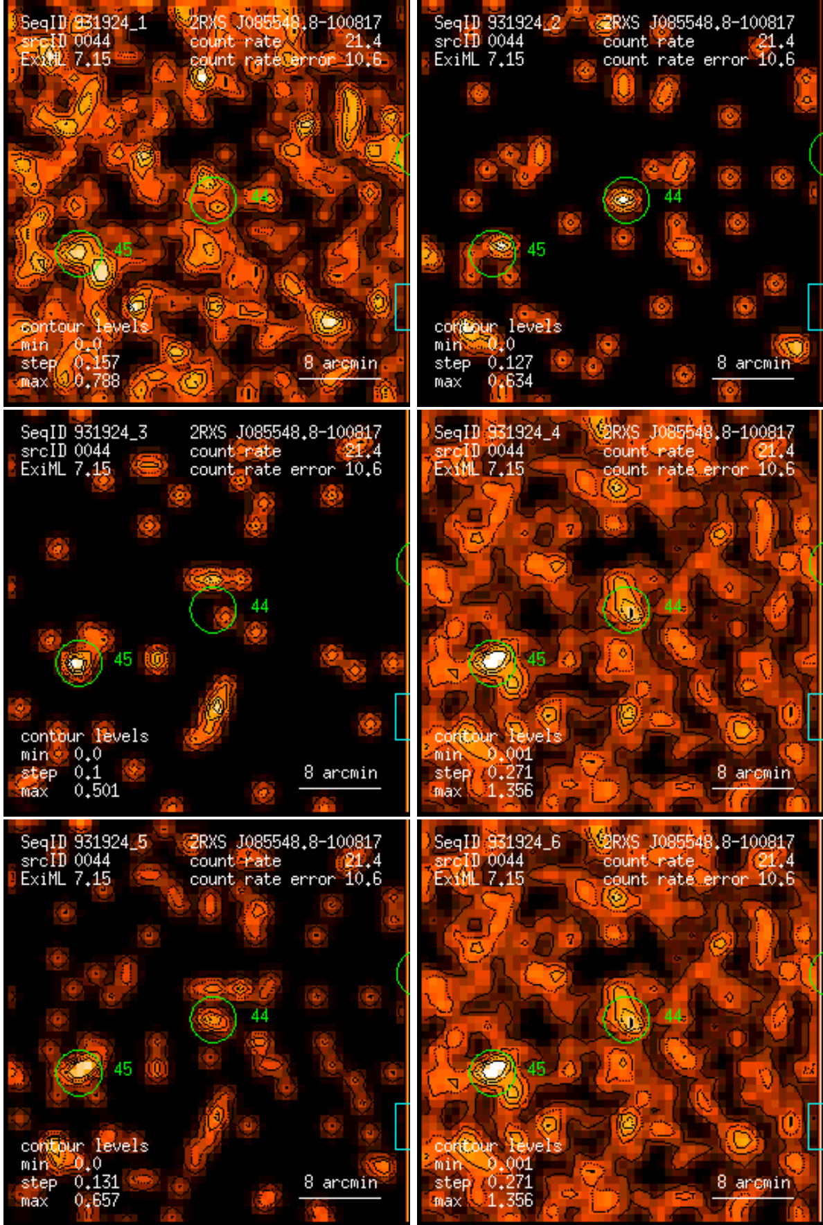
Figure 44: RASS 931924: detection 0044: band rate images, Gaussian filter: (1) PSPC channels 11 – 41, (2) 52 – 90, (3) 91 – 201, (4) 11 – 235, (5) 52 – 201, (6) 11 – 201. Broad band rates in counts/ks. Band rate contour levels in counts/ks/arcmin 2 .
