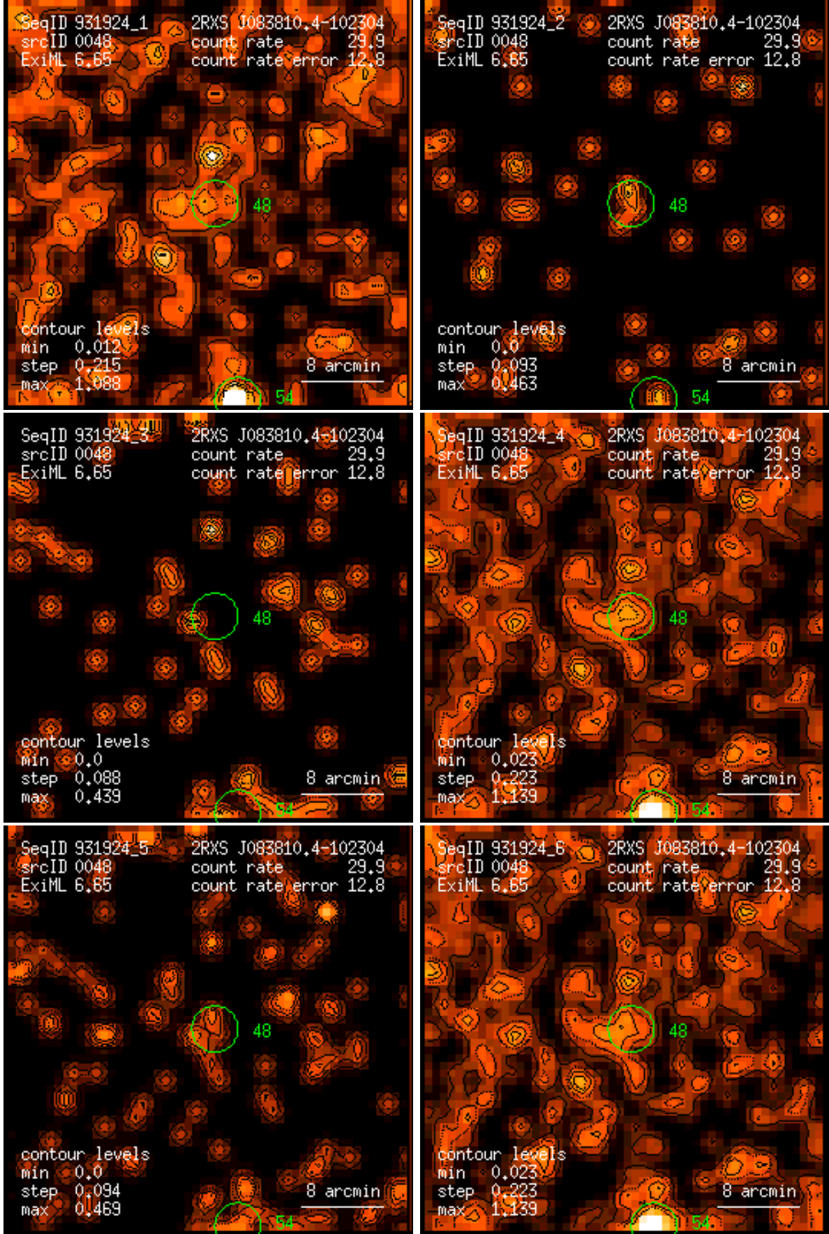
Figure 48: RASS 931924: detection 0048: band rate images, Gaussian filter: (1) PSPC channels 11 – 41, (2) 52 – 90, (3) 91 – 201, (4) 11 – 235, (5) 52 – 201, (6) 11 – 201. Broad band rates in counts/ks. Band rate contour levels in counts/ks/arcmin 2 .
