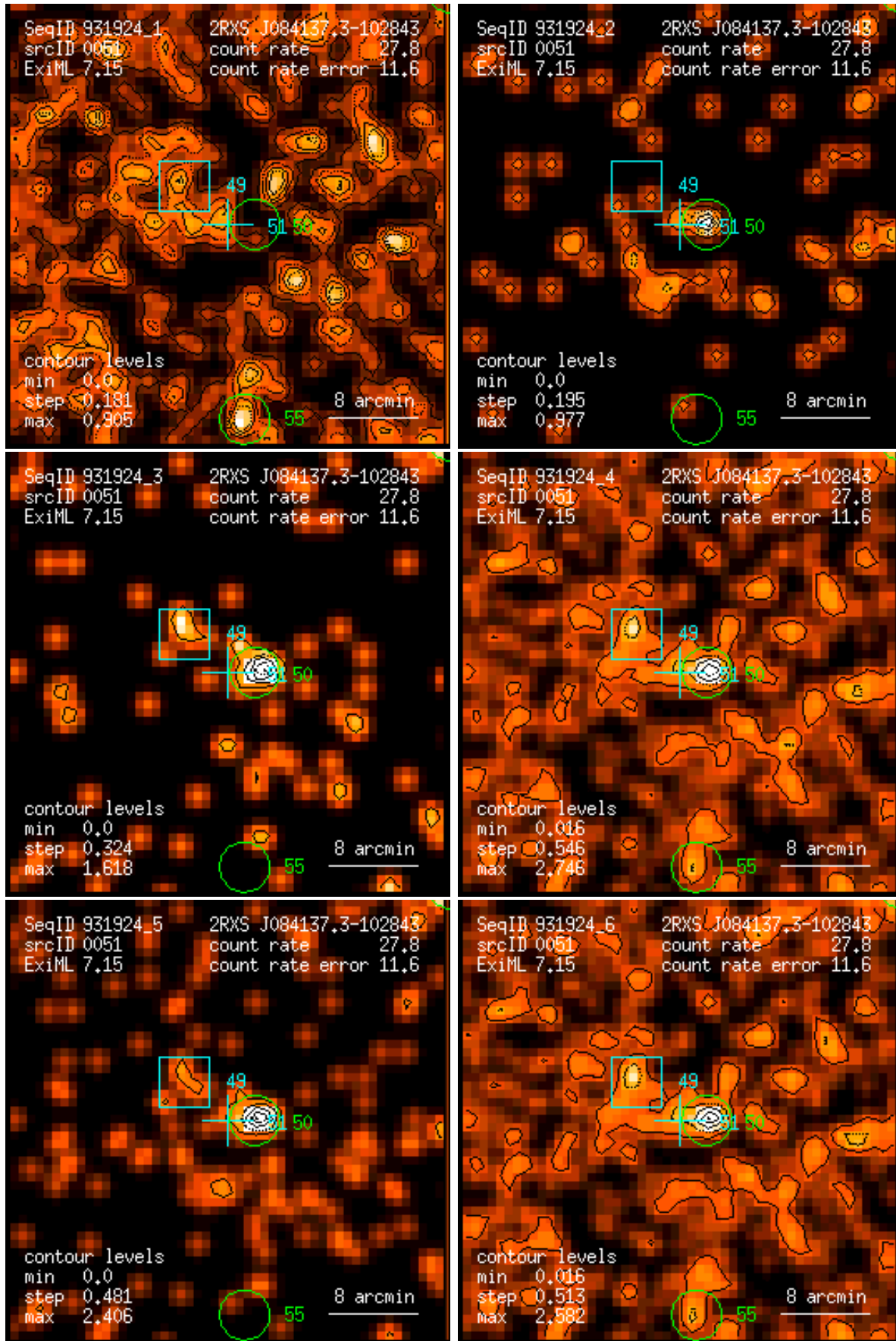
Figure 51: RASS 931924: detection 0051: band rate images, Gaussian filter: (1) PSPC channels 11 – 41, (2) 52 – 90, (3) 91 – 201, (4) 11 – 235, (5) 52 – 201, (6) 11 – 201. Broad band rates in counts/ks. Band rate contour levels in counts/ks/arcmin 2 .
