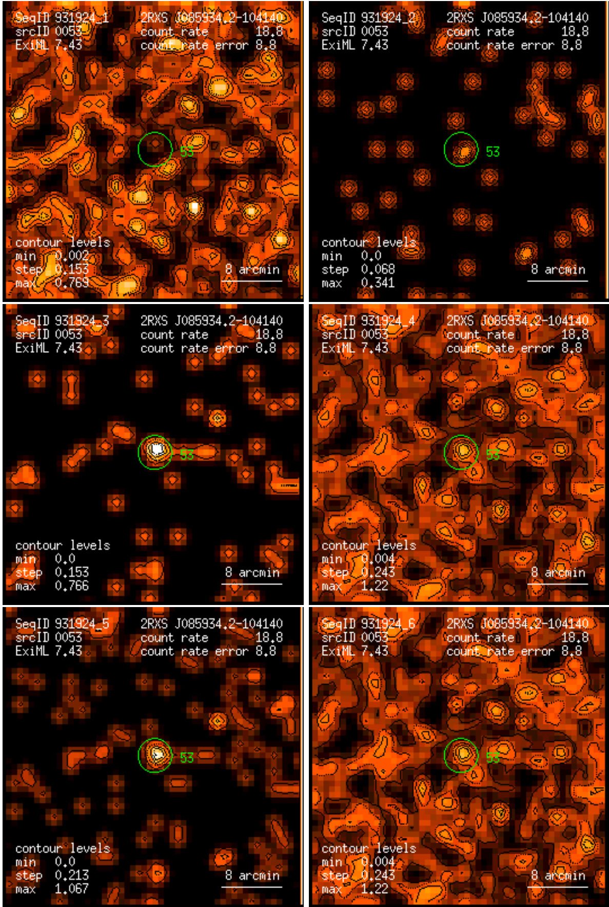
Figure 53: RASS 931924: detection 0053: band rate images, Gaussian filter: (1) PSPC channels 11 – 41, (2) 52 – 90, (3) 91 – 201, (4) 11 – 235, (5) 52 – 201, (6) 11 – 201. Broad band rates in counts/ks. Band rate contour levels in counts/ks/arcmin 2 .
