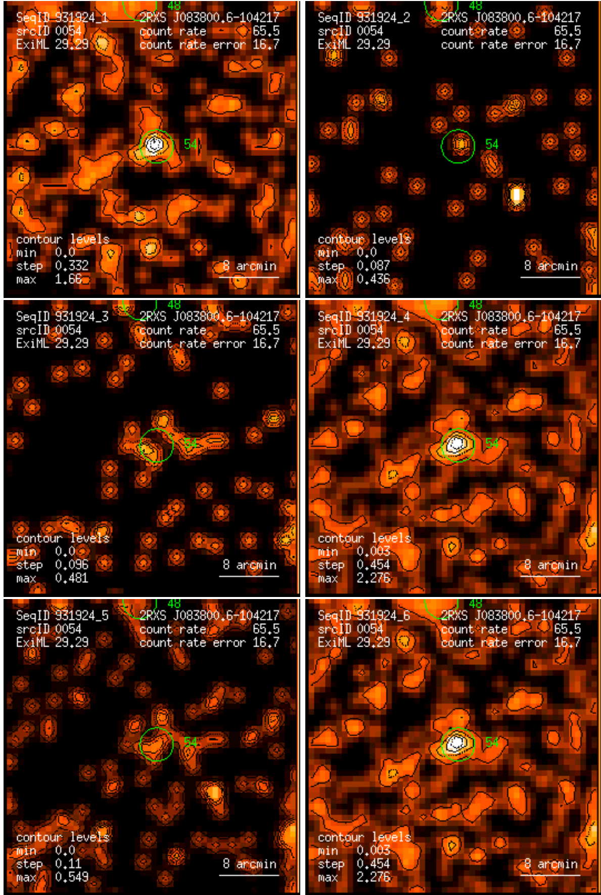
Figure 54: RASS 931924: detection 0054: band rate images, Gaussian filter: (1) PSPC channels 11 – 41, (2) 52 – 90, (3) 91 – 201, (4) 11 – 235, (5) 52 – 201, (6) 11 – 201. Broad band rates in counts/ks. Band rate contour levels in counts/ks/arcmin 2 .
