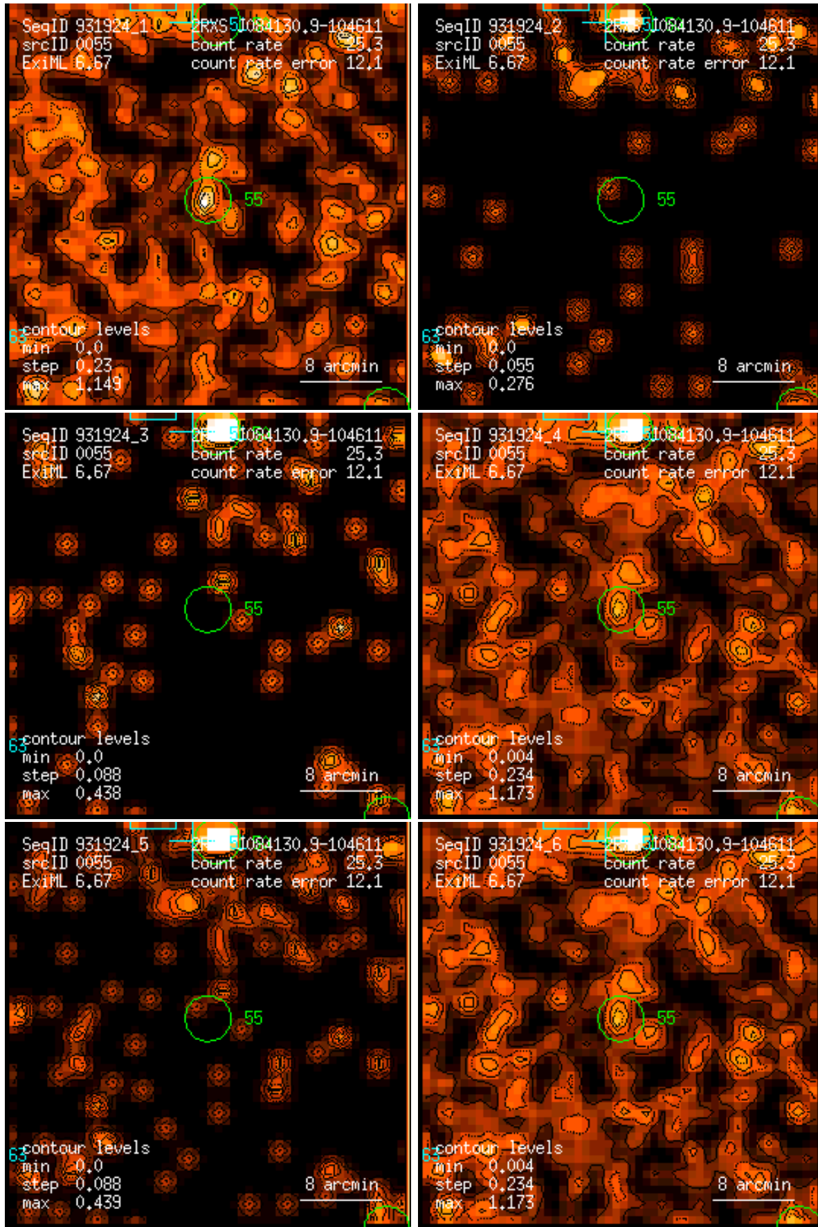
Figure 55: RASS 931924: detection 0055: band rate images, Gaussian filter: (1) PSPC channels 11 – 41, (2) 52 – 90, (3) 91 – 201, (4) 11 – 235, (5) 52 – 201, (6) 11 – 201. Broad band rates in counts/ks. Band rate contour levels in counts/ks/arcmin 2 .
