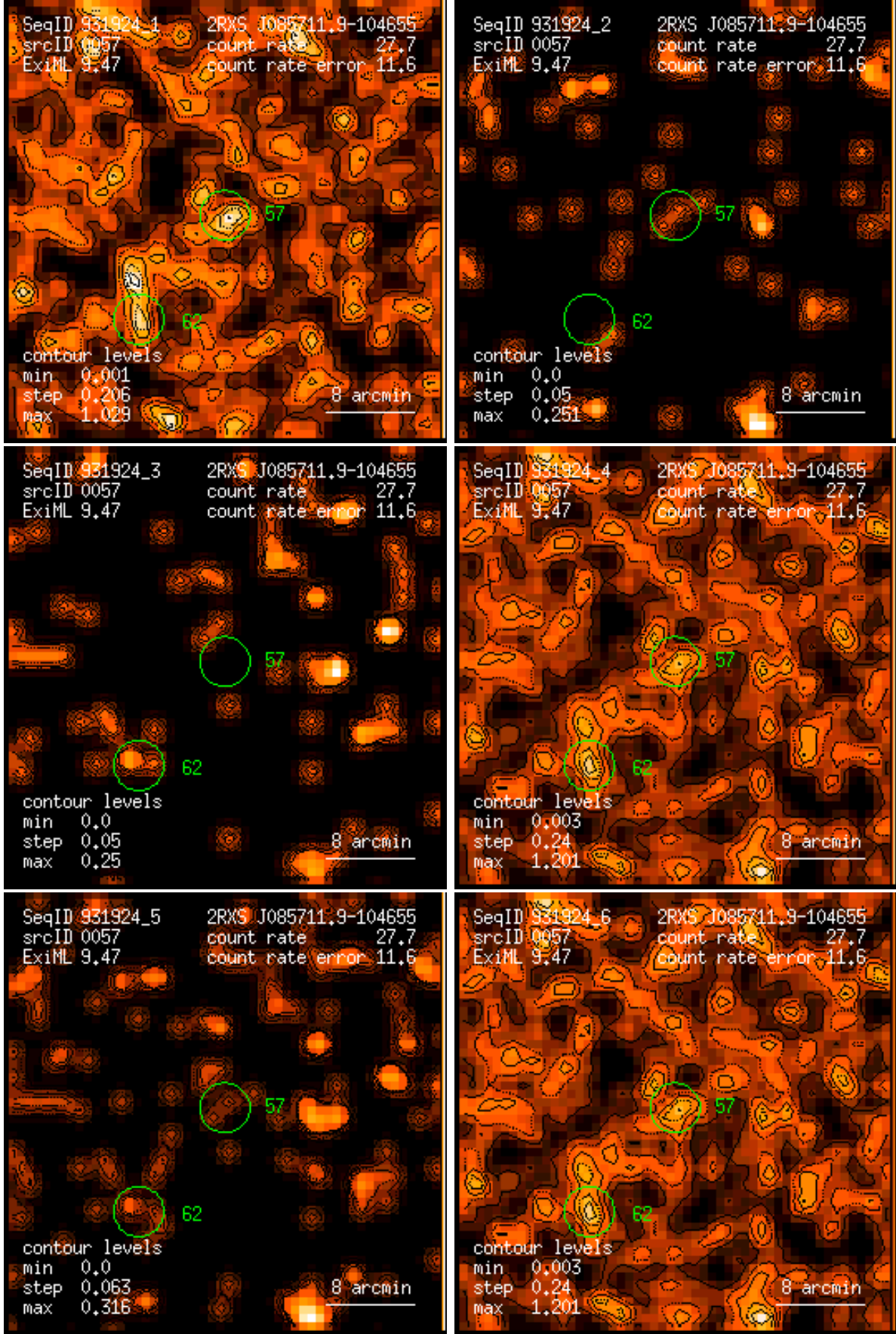
Figure 57: RASS 931924: detection 0057: band rate images, Gaussian filter: (1) PSPC channels 11 – 41, (2) 52 – 90, (3) 91 – 201, (4) 11 – 235, (5) 52 – 201, (6) 11 – 201. Broad band rates in counts/ks. Band rate contour levels in counts/ks/arcmin 2 .
