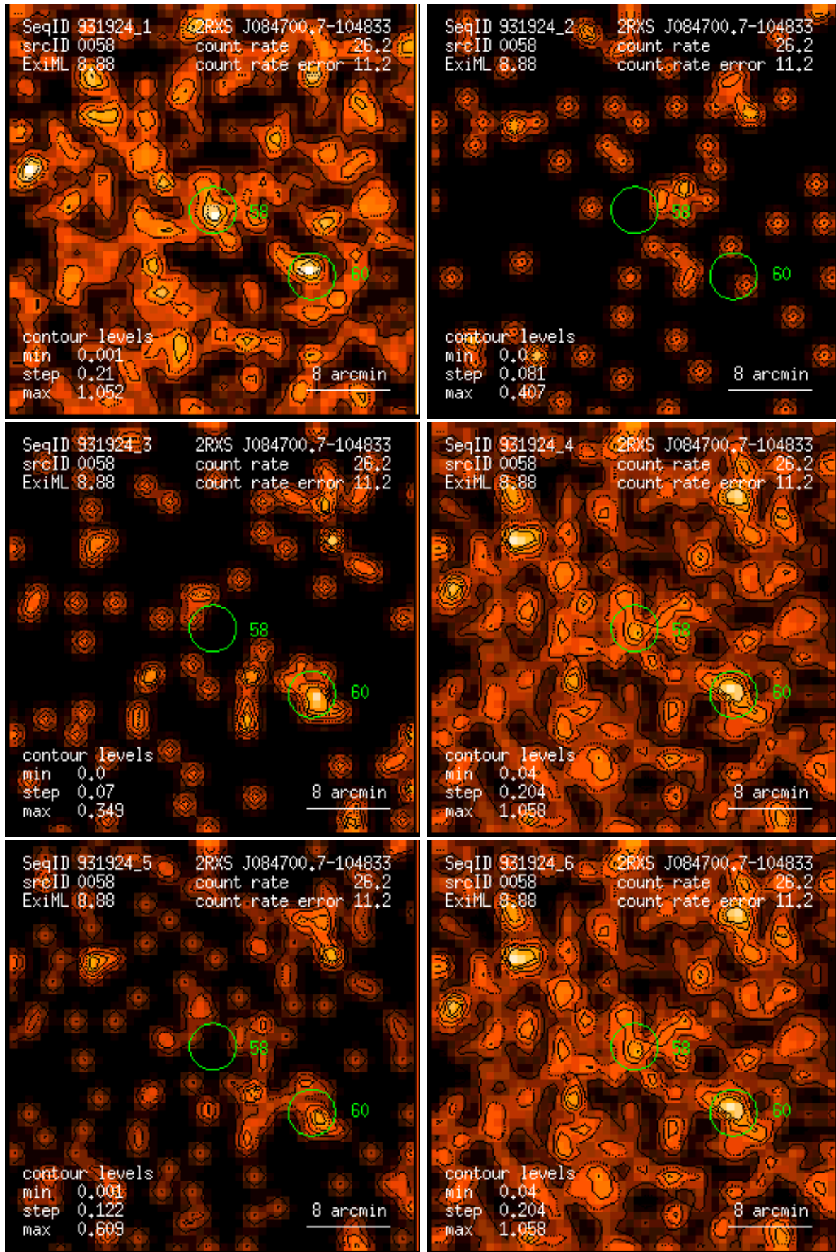
Figure 58: RASS 931924: detection 0058: band rate images, Gaussian filter: (1) PSPC channels 11 – 41, (2) 52 – 90, (3) 91 – 201, (4) 11 – 235, (5) 52 – 201, (6) 11 – 201. Broad band rates in counts/ks. Band rate contour levels in counts/ks/arcmin 2 .
